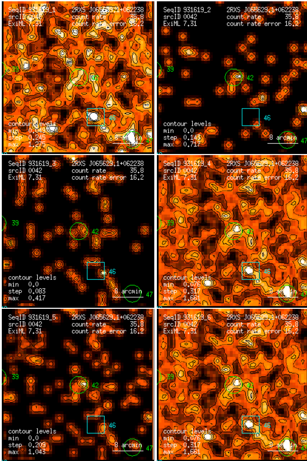
Figure 42: RASS 931619: detection 0042: band rate images, Gaussian filter: (1) PSPC channels 11 – 41, (2) 52 – 90, (3) 91 – 201, (4) 11 – 235, (5) 52 – 201, (6) 11 – 201. Broad band rates in counts/ks. Band rate contour levels in counts/ks/arcmin 2 .
