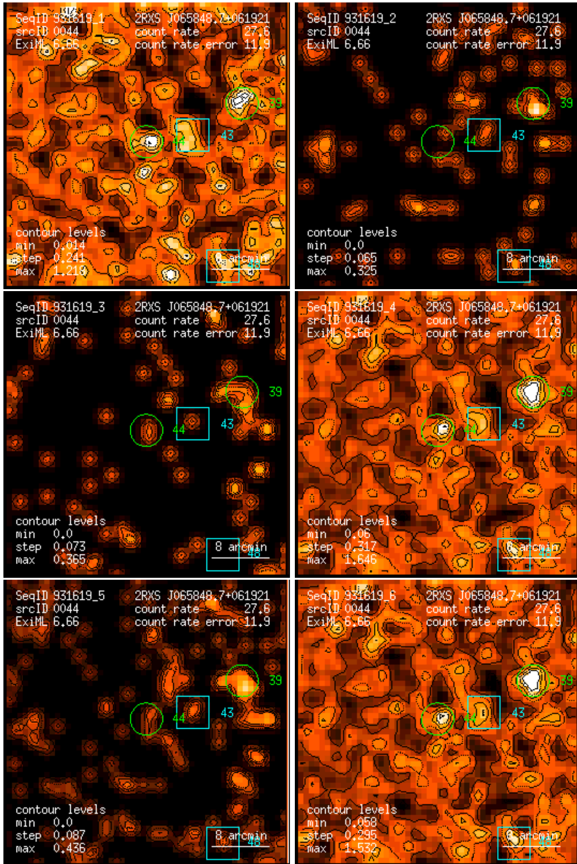
Figure 44: RASS 931619: detection 0044: band rate images, Gaussian filter: (1) PSPC channels 11 – 41, (2) 52 – 90, (3) 91 – 201, (4) 11 – 235, (5) 52 – 201, (6) 11 – 201. Broad band rates in counts/ks. Band rate contour levels in counts/ks/arcmin 2 .
