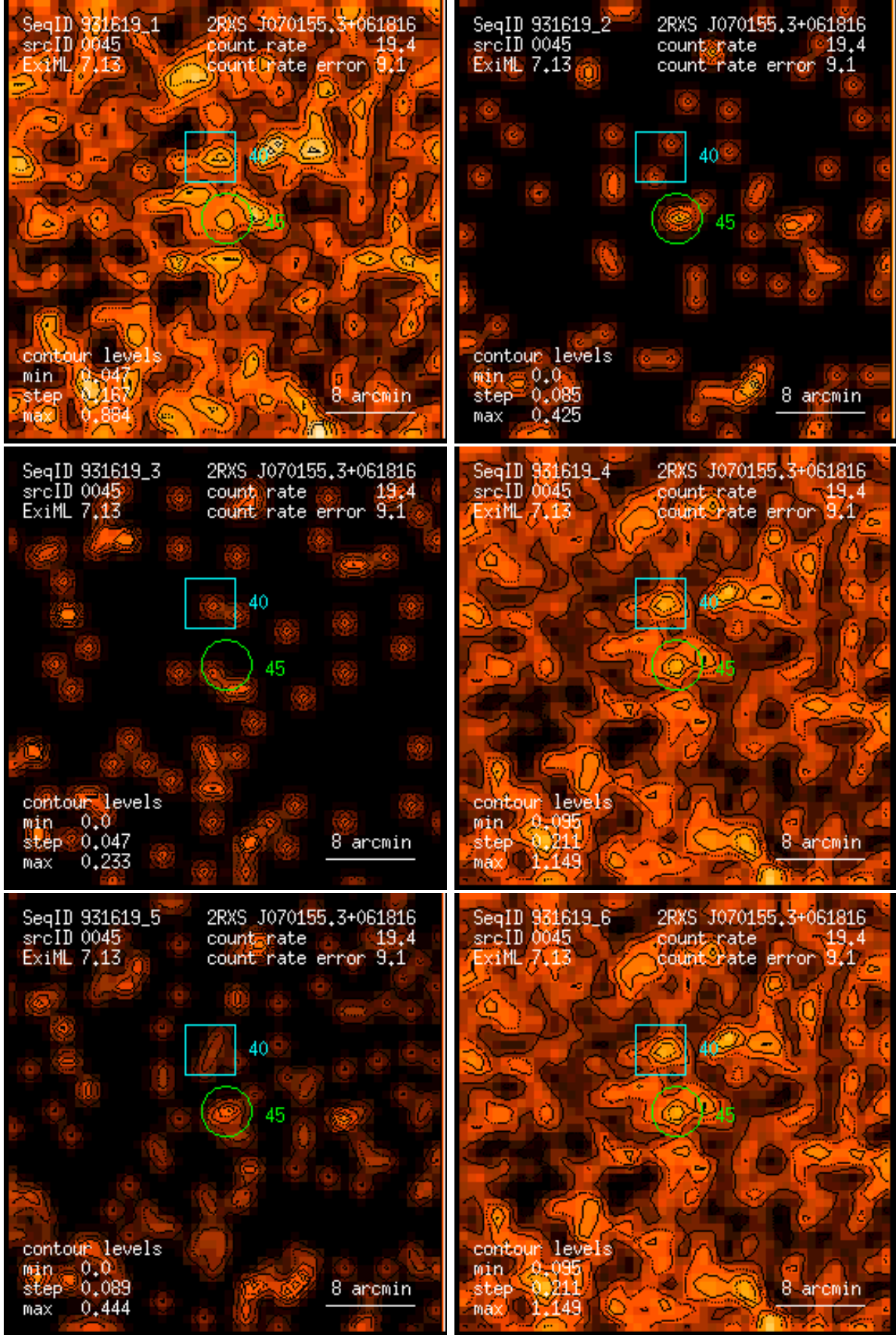
Figure 45: RASS 931619: detection 0045: band rate images, Gaussian filter: (1) PSPC channels 11 – 41, (2) 52 – 90, (3) 91 – 201, (4) 11 – 235, (5) 52 – 201, (6) 11 – 201. Broad band rates in counts/ks. Band rate contour levels in counts/ks/arcmin 2 .
