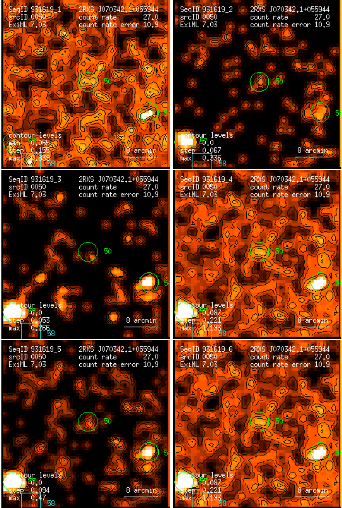
Figure 50: RASS 931619: detection 0050: band rate images, Gaussian filter: (1) PSPC channels 11 – 41, (2) 52 – 90, (3) 91 – 201, (4) 11 – 235, (5) 52 – 201, (6) 11 – 201. Broad band rates in counts/ks. Band rate contour levels in counts/ks/arcmin 2 .
