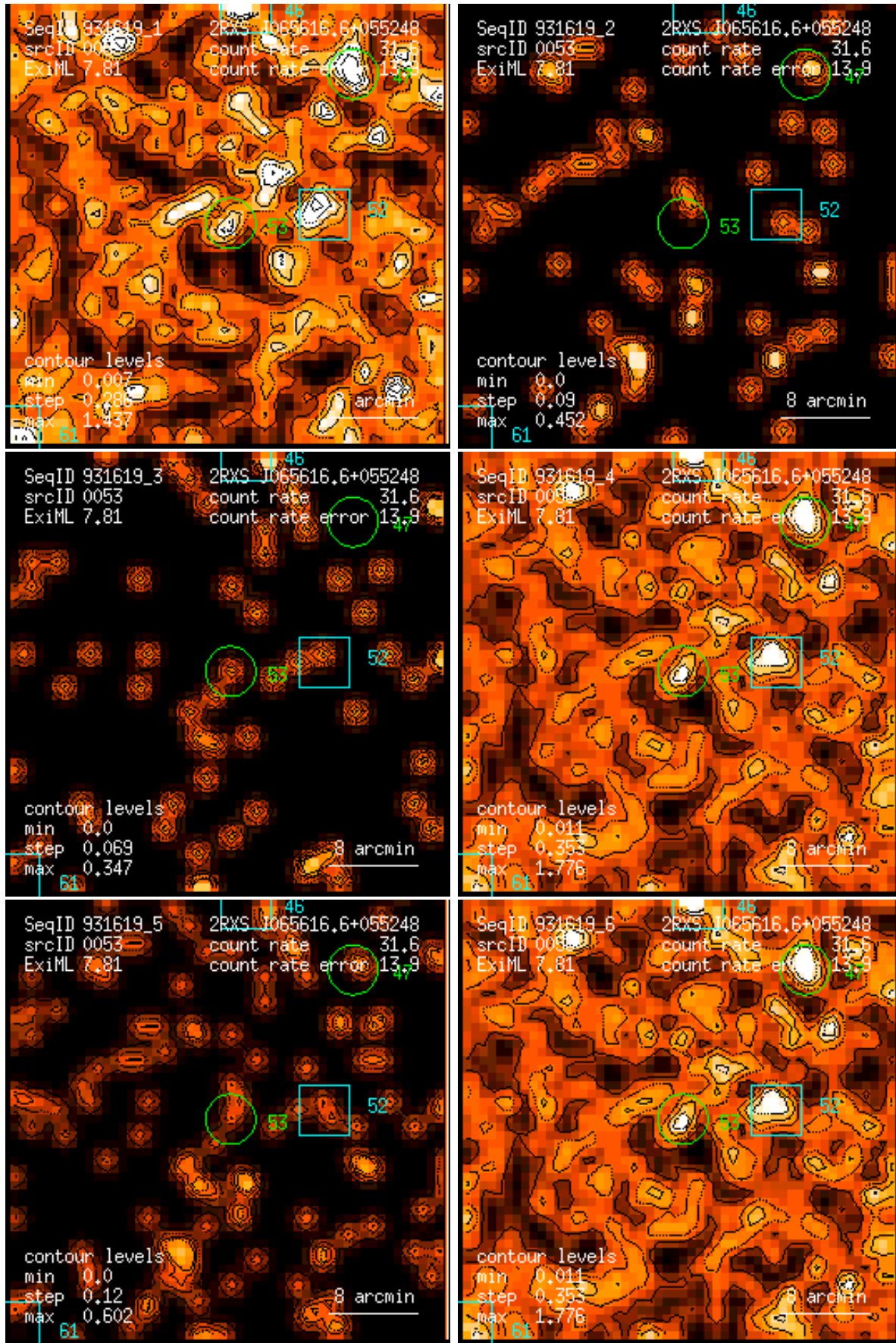
Figure 53: RASS 931619: detection 0053: band rate images, Gaussian filter: (1) PSPC channels 11 – 41, (2) 52 – 90, (3) 91 – 201, (4) 11 – 235, (5) 52 – 201, (6) 11 – 201. Broad band rates in counts/ks. Band rate contour levels in counts/ks/arcmin 2 .
