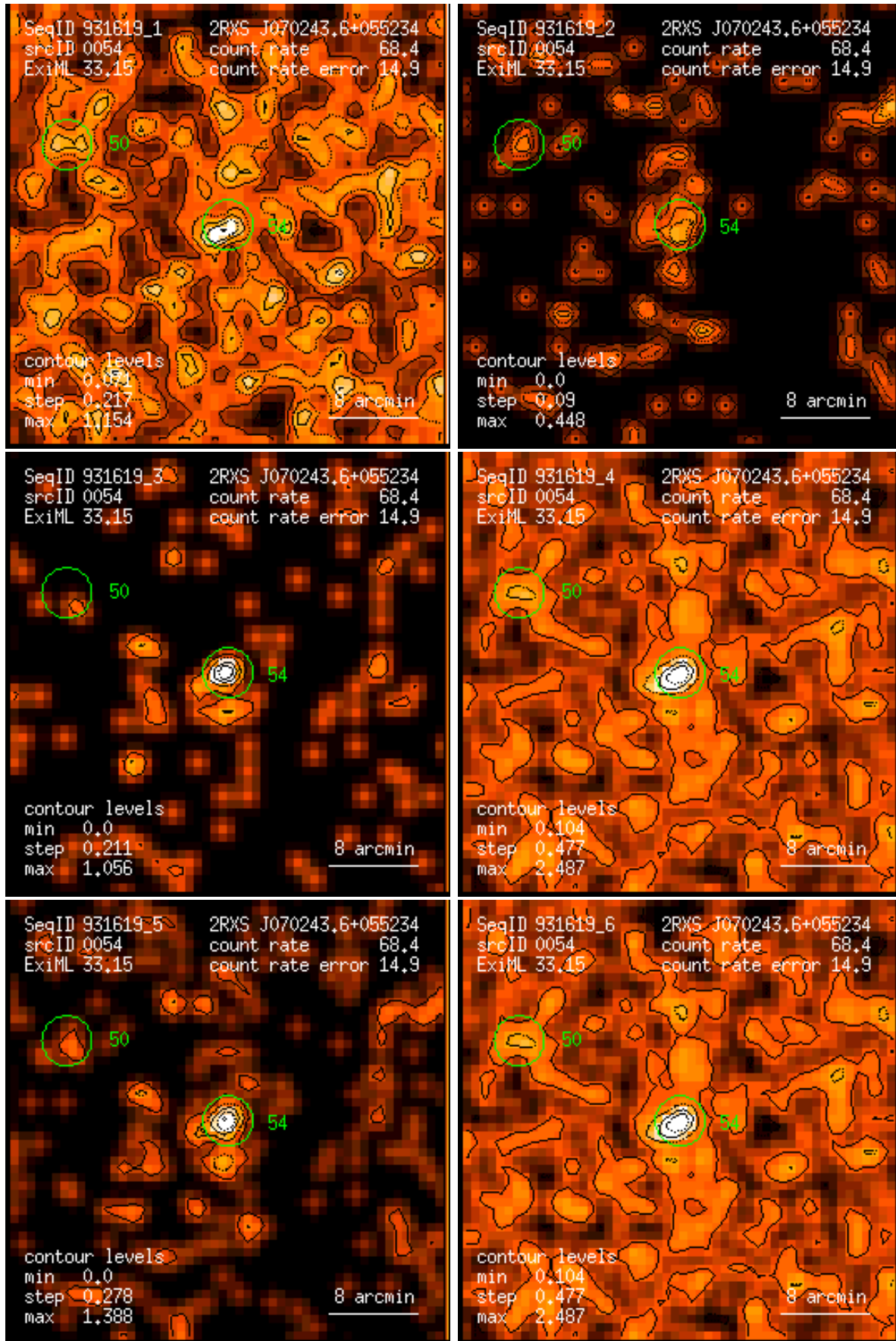
Figure 54: RASS 931619: detection 0054: band rate images, Gaussian filter: (1) PSPC channels 11 – 41, (2) 52 – 90, (3) 91 – 201, (4) 11 – 235, (5) 52 – 201, (6) 11 – 201. Broad band rates in counts/ks. Band rate contour levels in counts/ks/arcmin 2 .
