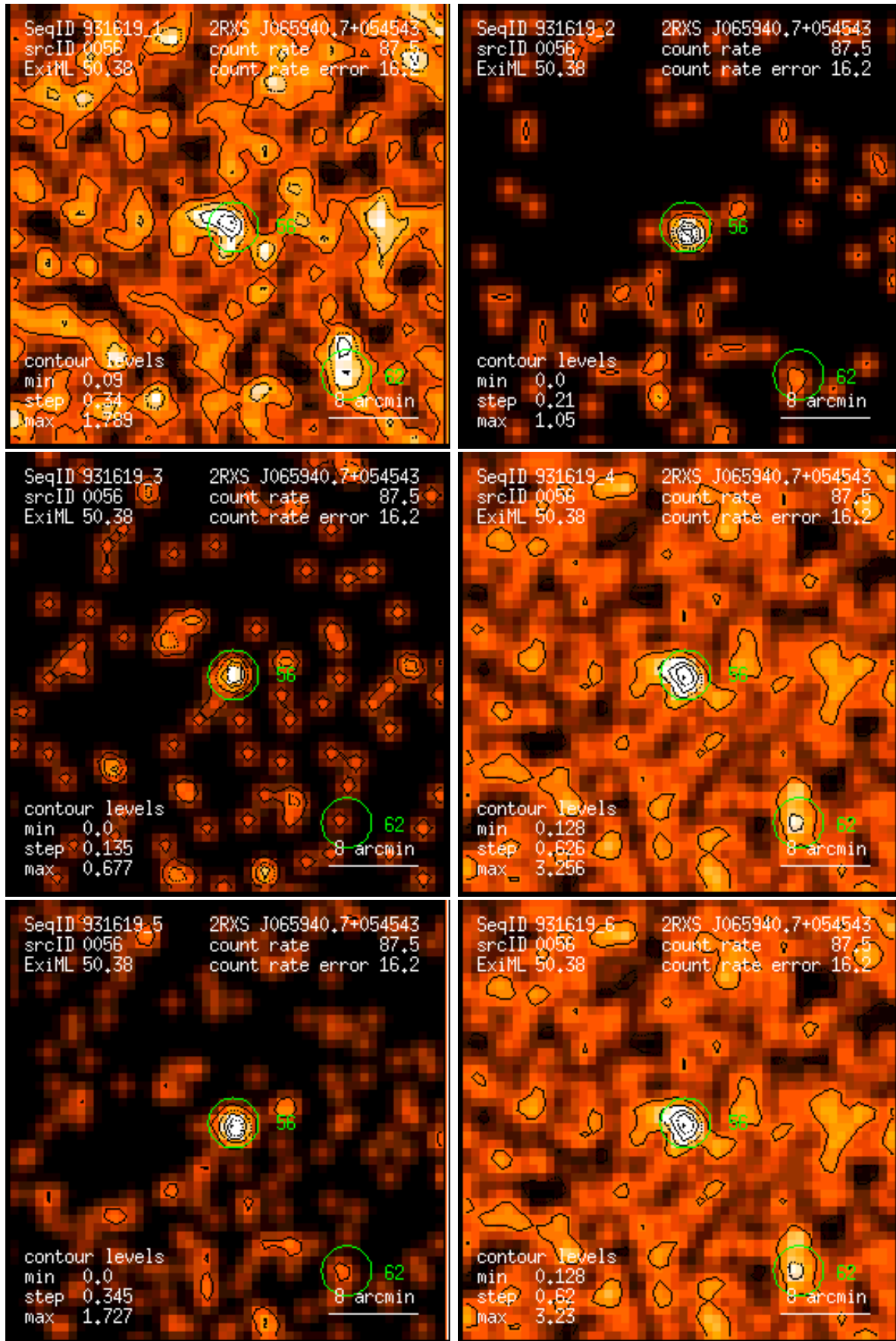
Figure 56: RASS 931619: detection 0056: band rate images, Gaussian filter: (1) PSPC channels 11 – 41, (2) 52 – 90, (3) 91 – 201, (4) 11 – 235, (5) 52 – 201, (6) 11 – 201. Broad band rates in counts/ks. Band rate contour levels in counts/ks/arcmin 2 .
