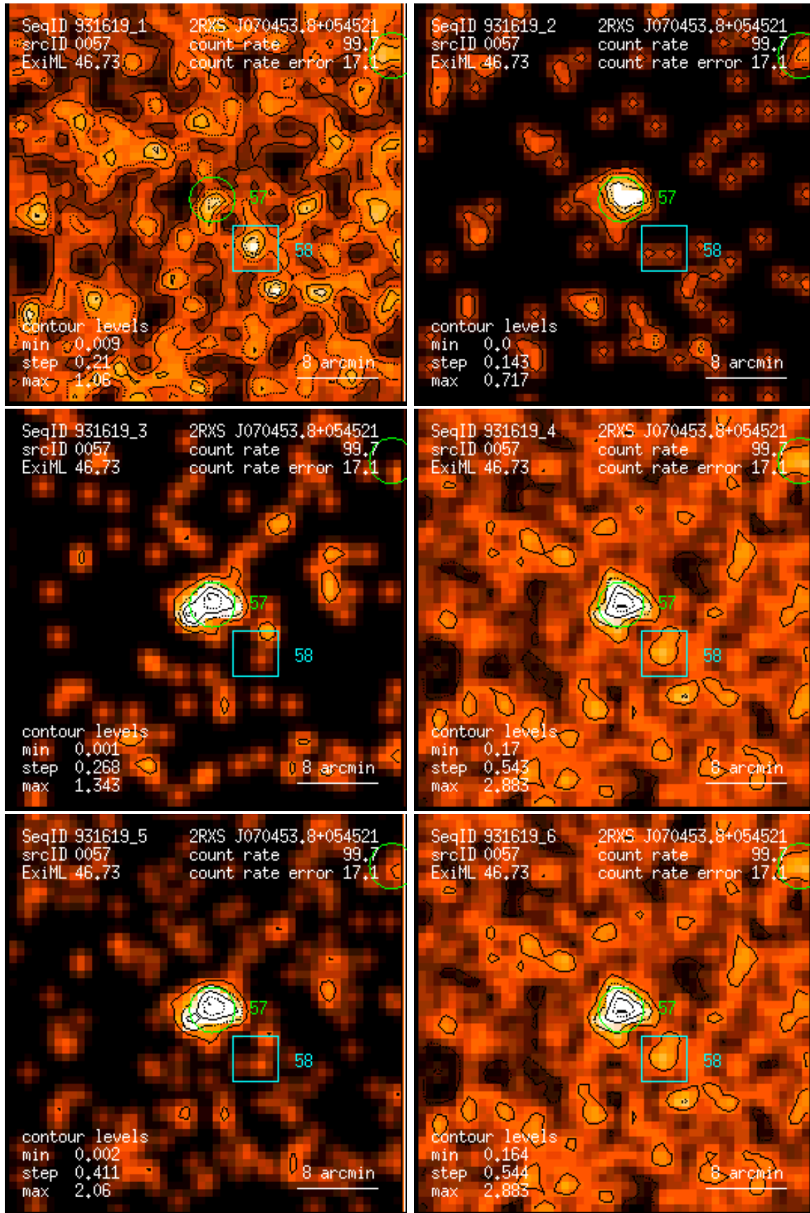
Figure 57: RASS 931619: detection 0057: band rate images, Gaussian filter: (1) PSPC channels 11 – 41, (2) 52 – 90, (3) 91 – 201, (4) 11 – 235, (5) 52 – 201, (6) 11 – 201. Broad band rates in counts/ks. Band rate contour levels in counts/ks/arcmin 2 .
