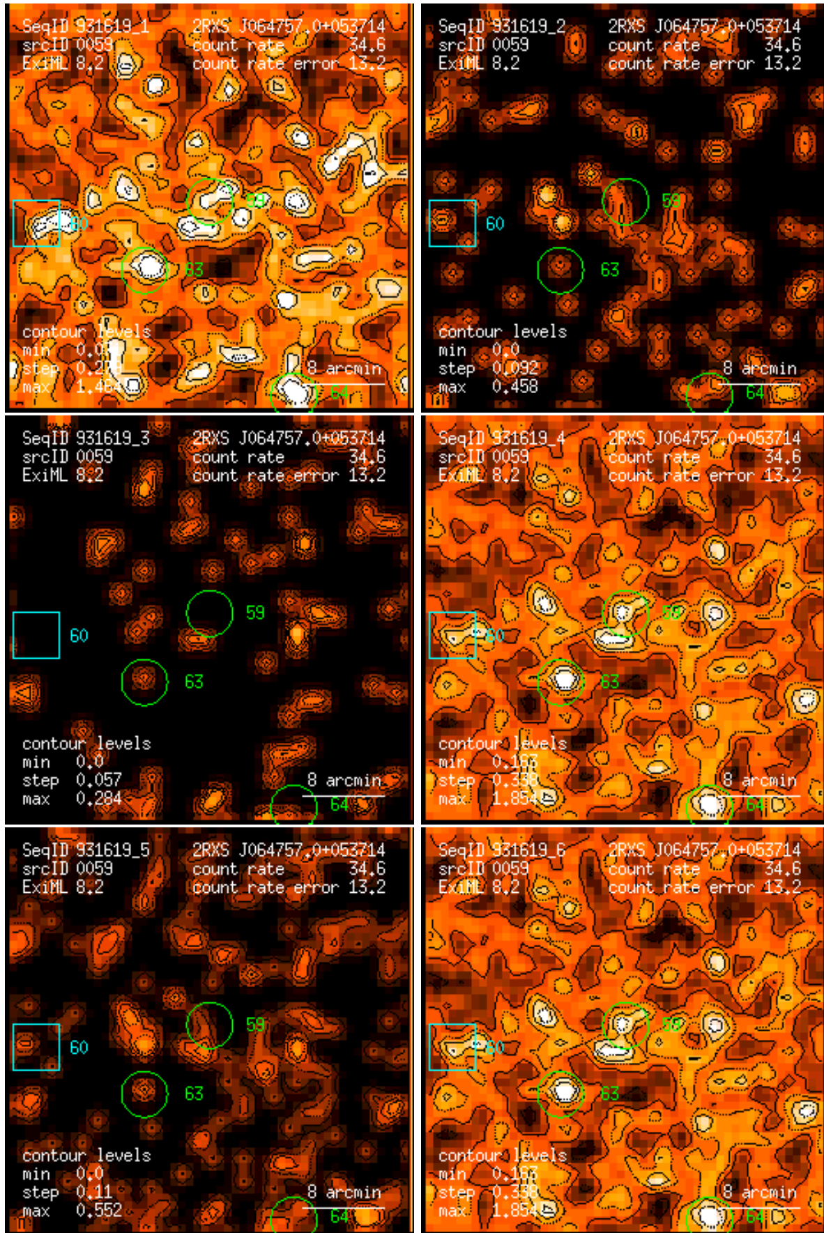
Figure 59: RASS 931619: detection 0059: band rate images, Gaussian filter: (1) PSPC channels 11 – 41, (2) 52 – 90, (3) 91 – 201, (4) 11 – 235, (5) 52 – 201, (6) 11 – 201. Broad band rates in counts/ks. Band rate contour levels in counts/ks/arcmin 2 .
