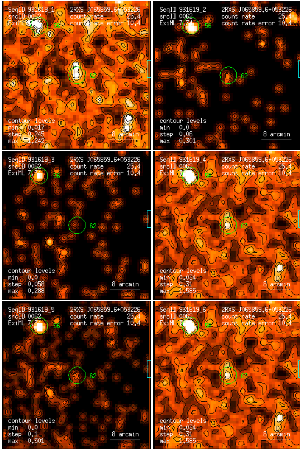
Figure 62: RASS 931619: detection 0062: band rate images, Gaussian filter: (1) PSPC channels 11 – 41, (2) 52 – 90, (3) 91 – 201, (4) 11 – 235, (5) 52 – 201, (6) 11 – 201. Broad band rates in counts/ks. Band rate contour levels in counts/ks/arcmin 2 .
