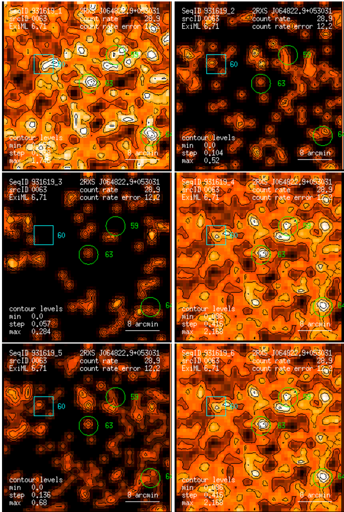
Figure 63: RASS 931619: detection 0063: band rate images, Gaussian filter: (1) PSPC channels 11 – 41, (2) 52 – 90, (3) 91 – 201, (4) 11 – 235, (5) 52 – 201, (6) 11 – 201. Broad band rates in counts/ks. Band rate contour levels in counts/ks/arcmin 2 .
