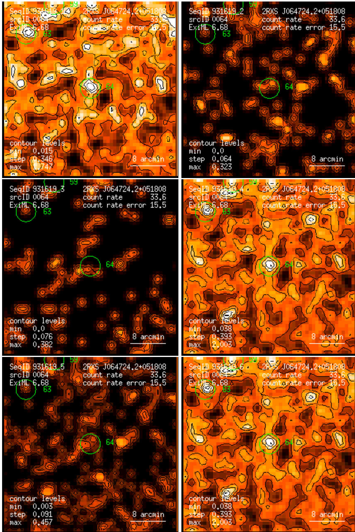
Figure 64: RASS 931619: detection 0064: band rate images, Gaussian filter: (1) PSPC channels 11 – 41, (2) 52 – 90, (3) 91 – 201, (4) 11 – 235, (5) 52 – 201, (6) 11 – 201. Broad band rates in counts/ks. Band rate contour levels in counts/ks/arcmin 2 .
