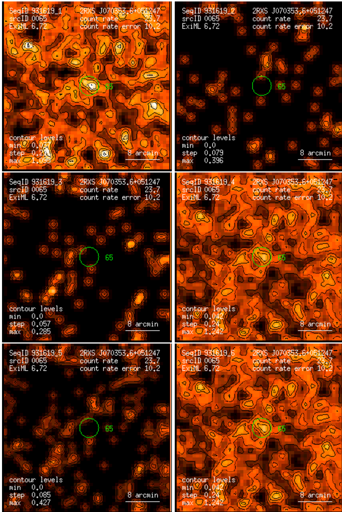
Figure 65: RASS 931619: detection 0065: band rate images, Gaussian filter: (1) PSPC channels 11 – 41, (2) 52 – 90, (3) 91 – 201, (4) 11 – 235, (5) 52 – 201, (6) 11 – 201. Broad band rates in counts/ks. Band rate contour levels in counts/ks/arcmin 2 .
