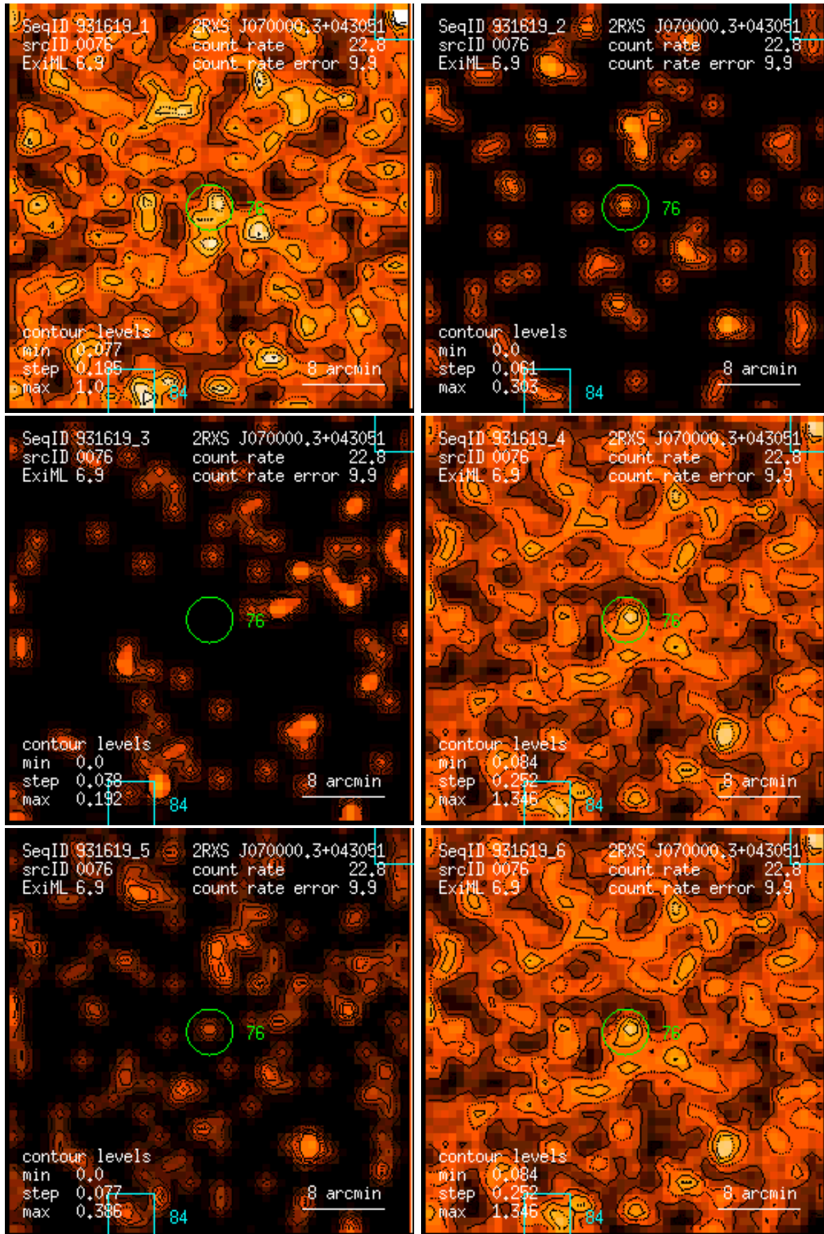
Figure 76: RASS 931619: detection 0076: band rate images, Gaussian filter: (1) PSPC channels 11 – 41, (2) 52 – 90, (3) 91 – 201, (4) 11 – 235, (5) 52 – 201, (6) 11 – 201. Broad band rates in counts/ks. Band rate contour levels in counts/ks/arcmin 2 .
