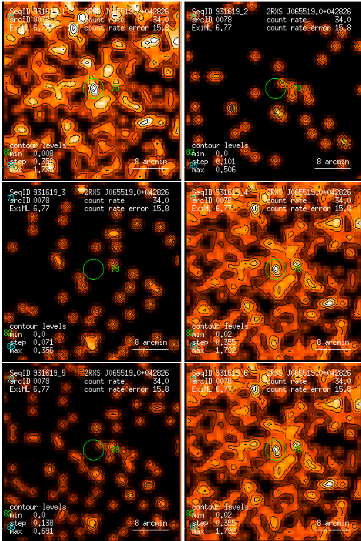
Figure 78: RASS 931619: detection 0078: band rate images, Gaussian filter: (1) PSPC channels 11 – 41, (2) 52 – 90, (3) 91 – 201, (4) 11 – 235, (5) 52 – 201, (6) 11 – 201. Broad band rates in counts/ks. Band rate contour levels in counts/ks/arcmin 2 .
