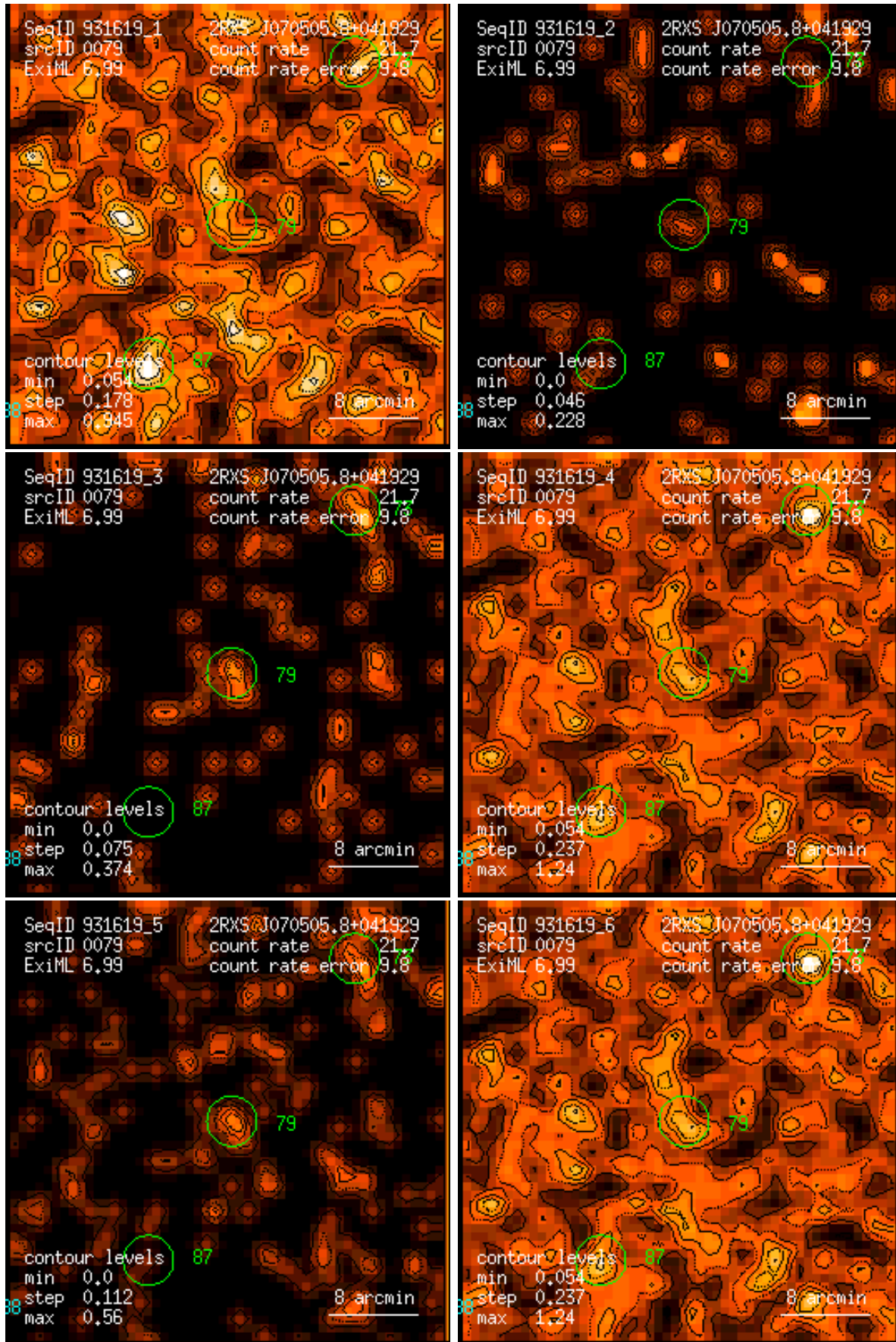
Figure 79: RASS 931619: detection 0079: band rate images, Gaussian filter: (1) PSPC channels 11 – 41, (2) 52 – 90, (3) 91 – 201, (4) 11 – 235, (5) 52 – 201, (6) 11 – 201. Broad band rates in counts/ks. Band rate contour levels in counts/ks/arcmin 2 .
