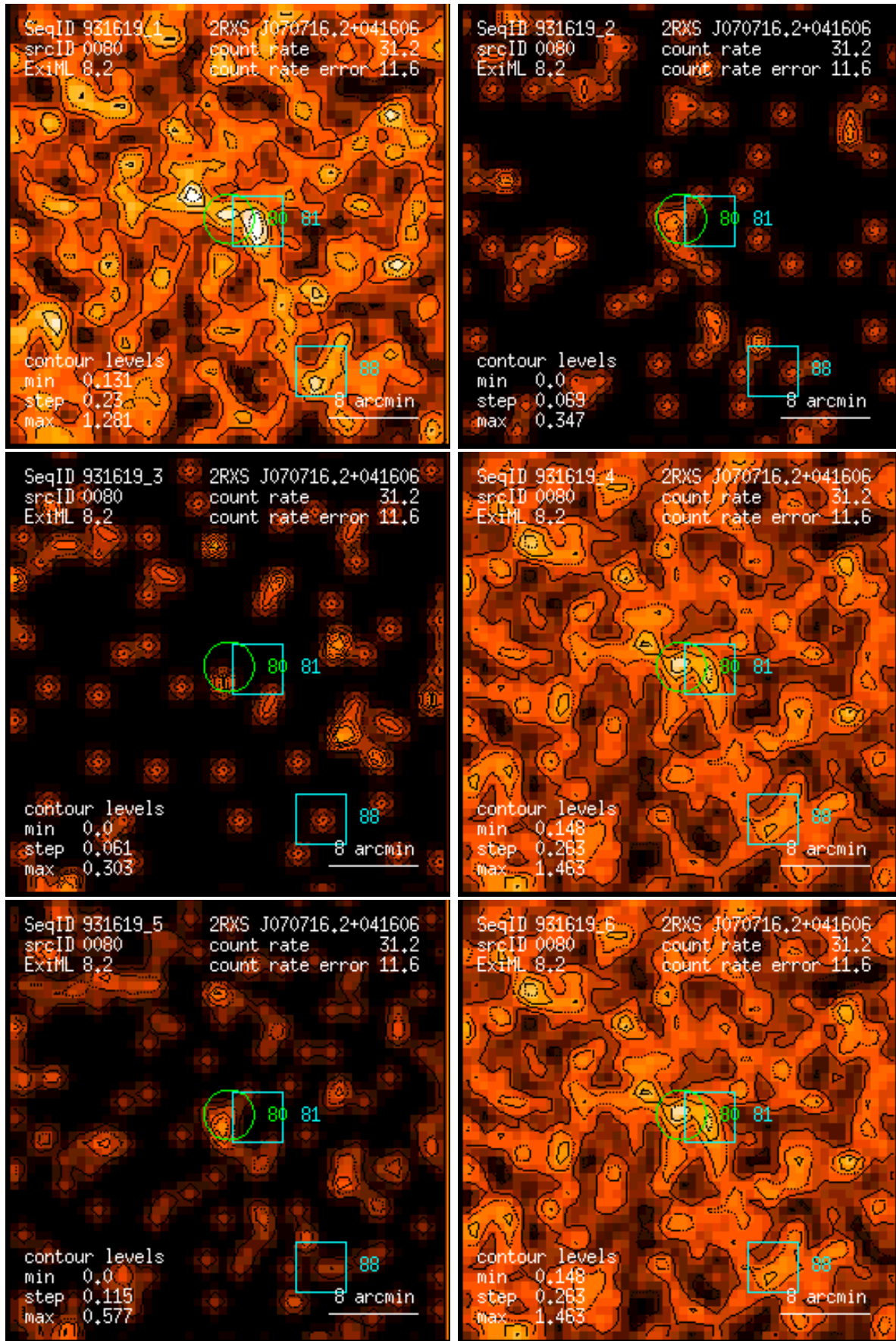
Figure 80: RASS 931619: detection 0080: band rate images, Gaussian filter: (1) PSPC channels 11 – 41, (2) 52 – 90, (3) 91 – 201, (4) 11 – 235, (5) 52 – 201, (6) 11 – 201. Broad band rates in counts/ks. Band rate contour levels in counts/ks/arcmin 2 .
