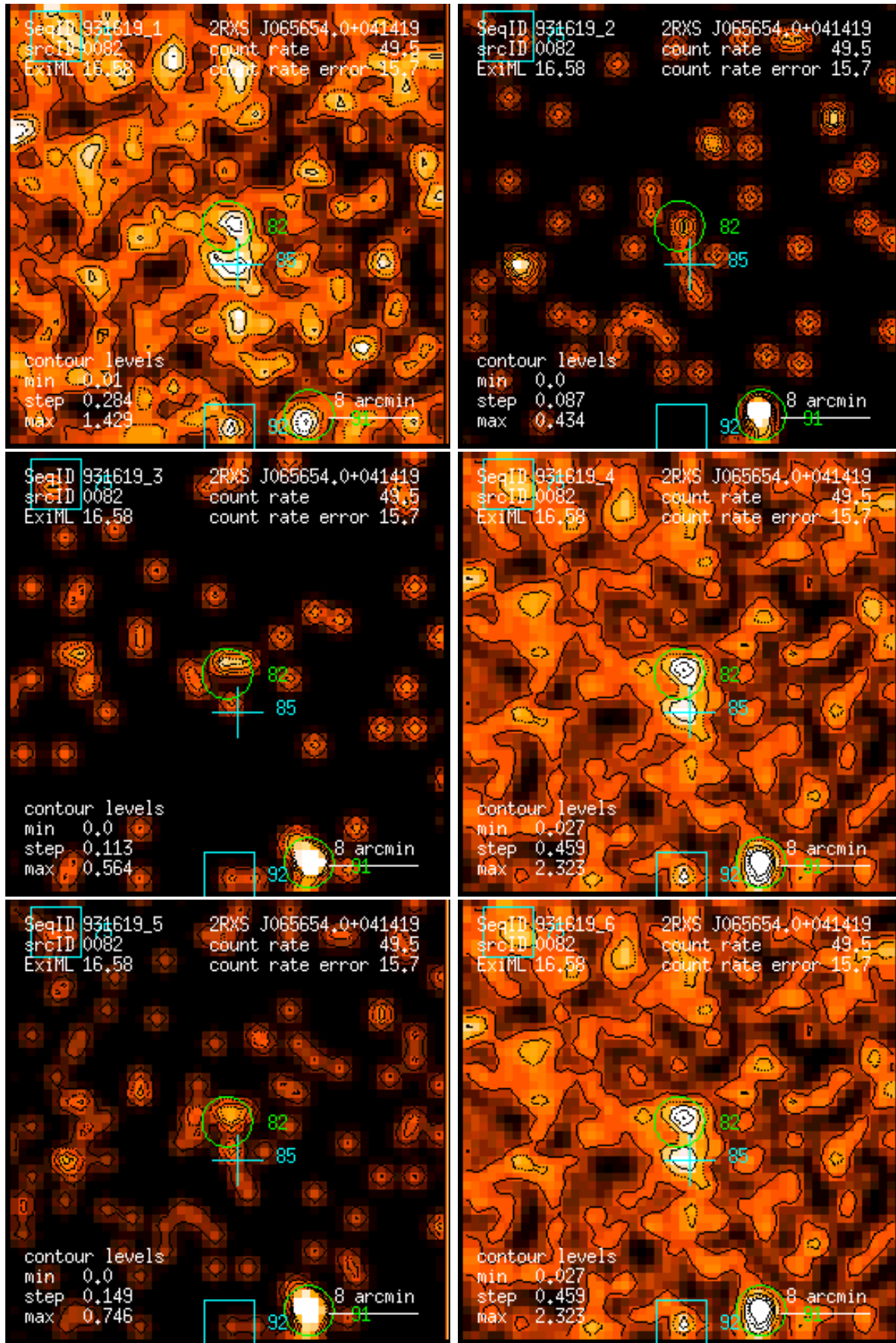
Figure 82: RASS 931619: detection 0082: band rate images, Gaussian filter: (1) PSPC channels 11 – 41, (2) 52 – 90, (3) 91 – 201, (4) 11 – 235, (5) 52 – 201, (6) 11 – 201. Broad band rates in counts/ks. Band rate contour levels in counts/ks/arcmin 2 .
