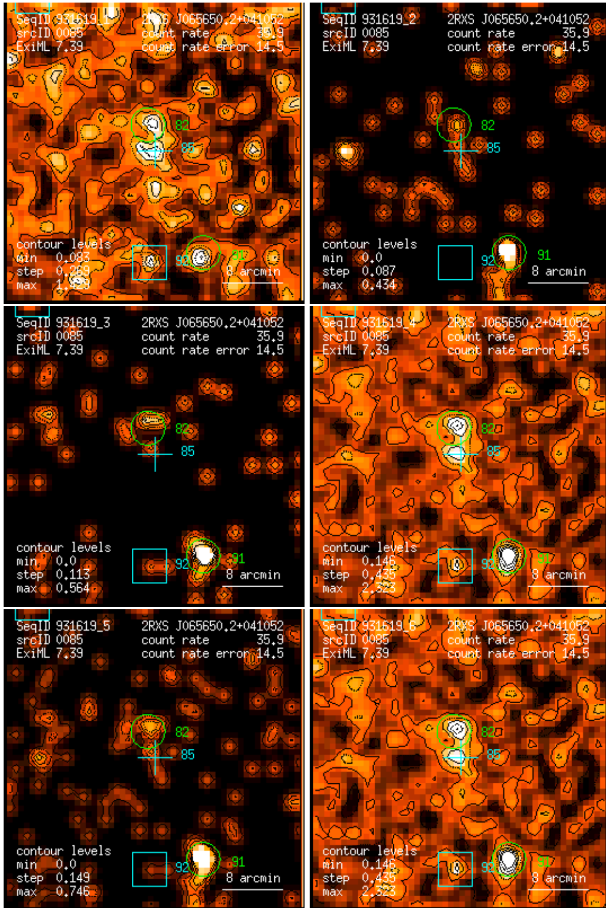
Figure 85: RASS 931619: detection 0085: band rate images, Gaussian filter: (1) PSPC channels 11 – 41, (2) 52 – 90, (3) 91 – 201, (4) 11 – 235, (5) 52 – 201, (6) 11 – 201. Broad band rates in counts/ks. Band rate contour levels in counts/ks/arcmin 2 .
