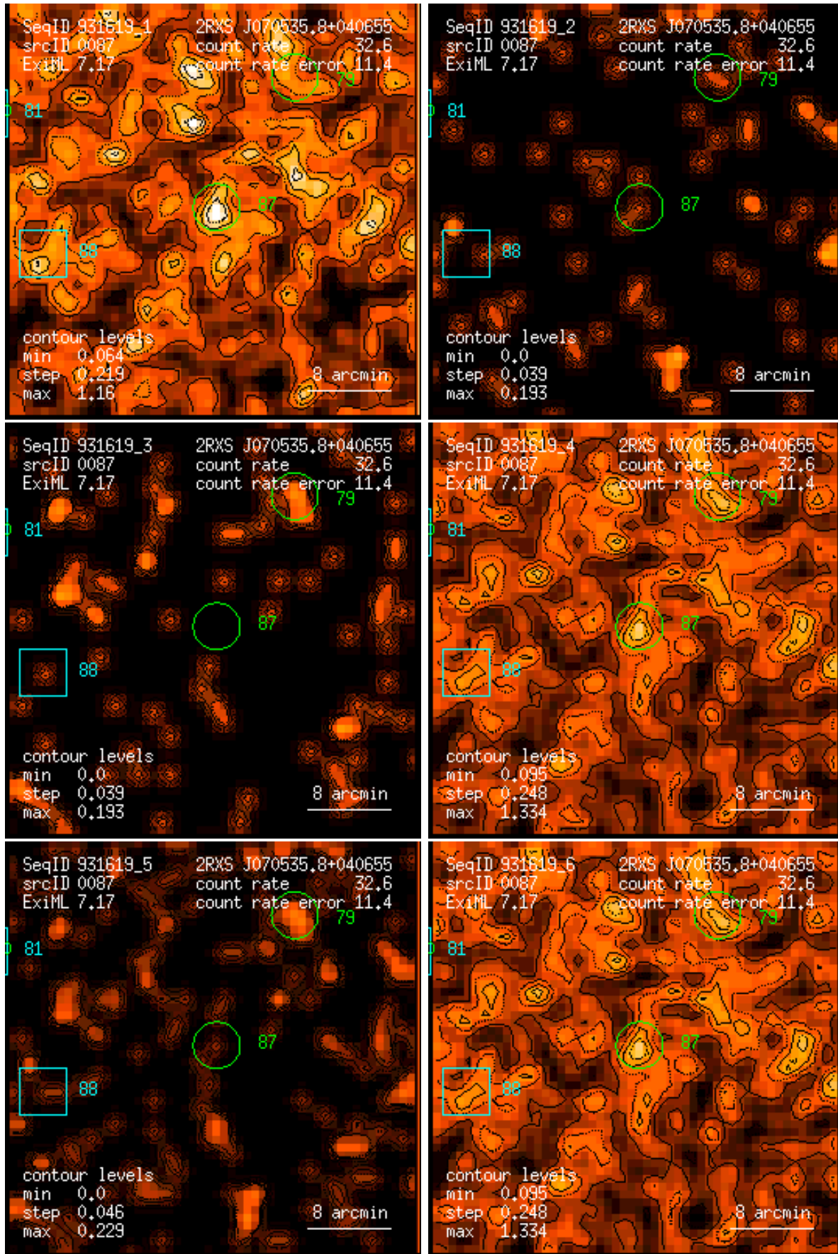
Figure 87: RASS 931619: detection 0087: band rate images, Gaussian filter: (1) PSPC channels 11 – 41, (2) 52 – 90, (3) 91 – 201, (4) 11 – 235, (5) 52 – 201, (6) 11 – 201. Broad band rates in counts/ks. Band rate contour levels in counts/ks/arcmin 2 .
