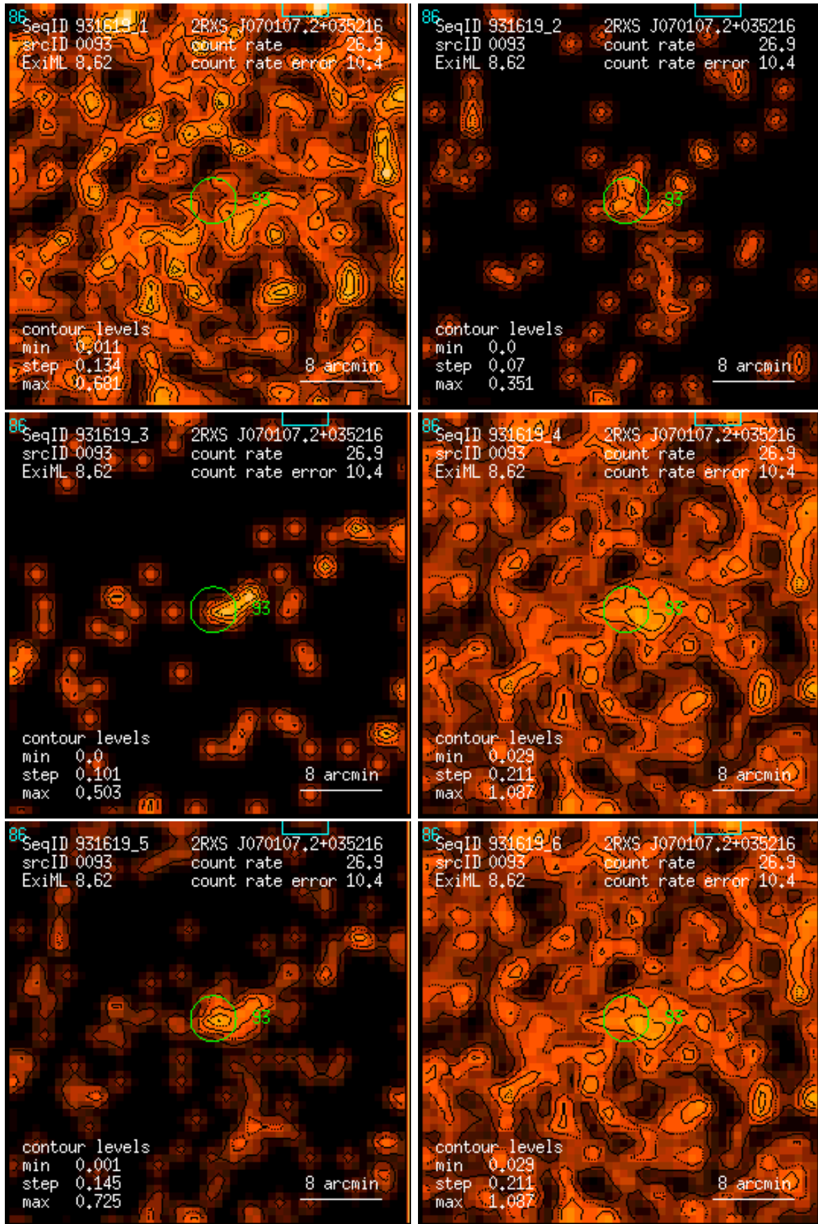
Figure 93: RASS 931619: detection 0093: band rate images, Gaussian filter: (1) PSPC channels 11 – 41, (2) 52 – 90, (3) 91 – 201, (4) 11 – 235, (5) 52 – 201, (6) 11 – 201. Broad band rates in counts/ks. Band rate contour levels in counts/ks/arcmin 2 .
