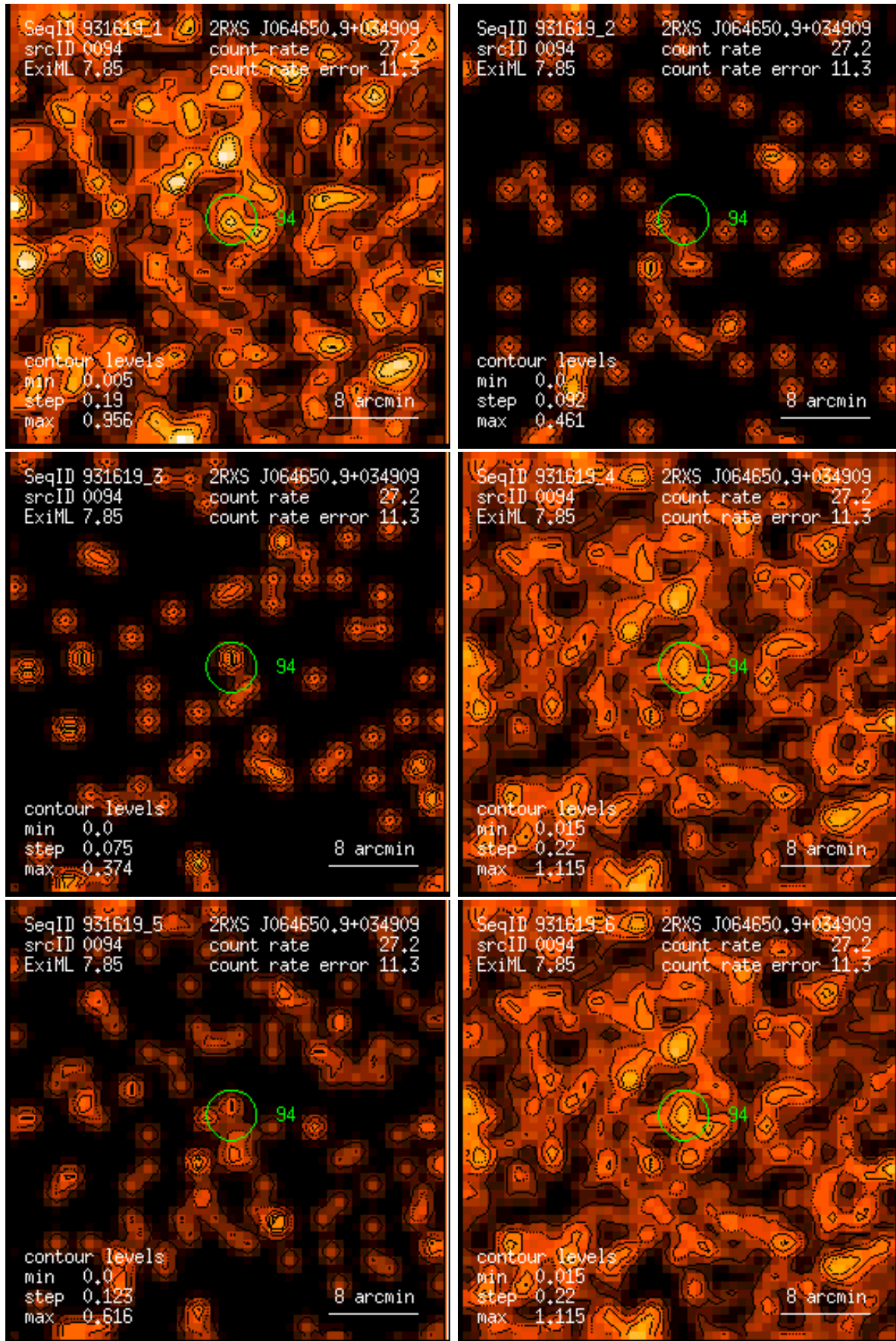
Figure 94: RASS 931619: detection 0094: band rate images, Gaussian filter: (1) PSPC channels 11 – 41, (2) 52 – 90, (3) 91 – 201, (4) 11 – 235, (5) 52 – 201, (6) 11 – 201. Broad band rates in counts/ks. Band rate contour levels in counts/ks/arcmin 2 .
