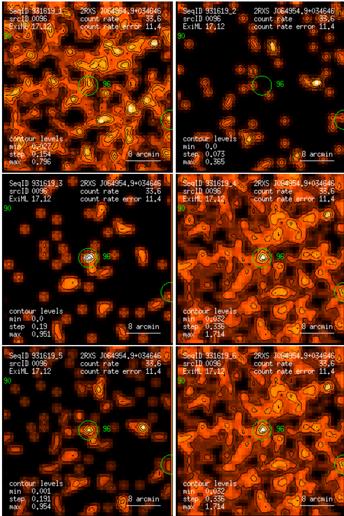
Figure 96: RASS 931619: detection 0096: band rate images, Gaussian filter: (1) PSPC channels 11 – 41, (2) 52 – 90, (3) 91 – 201, (4) 11 – 235, (5) 52 – 201, (6) 11 – 201. Broad band rates in counts/ks. Band rate contour levels in counts/ks/arcmin 2 .
