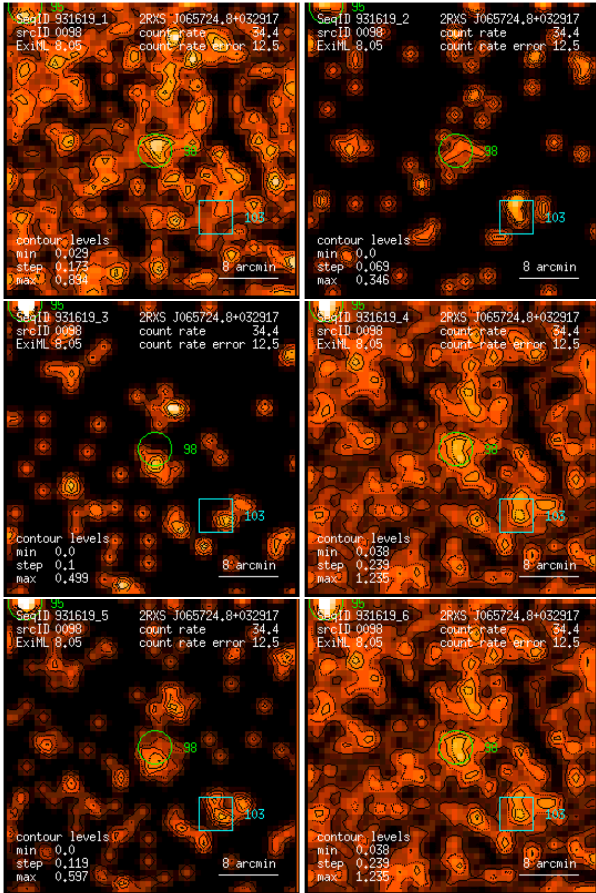
Figure 98: RASS 931619: detection 0098: band rate images, Gaussian filter: (1) PSPC channels 11 – 41, (2) 52 – 90, (3) 91 – 201, (4) 11 – 235, (5) 52 – 201, (6) 11 – 201. Broad band rates in counts/ks. Band rate contour levels in counts/ks/arcmin 2 .
