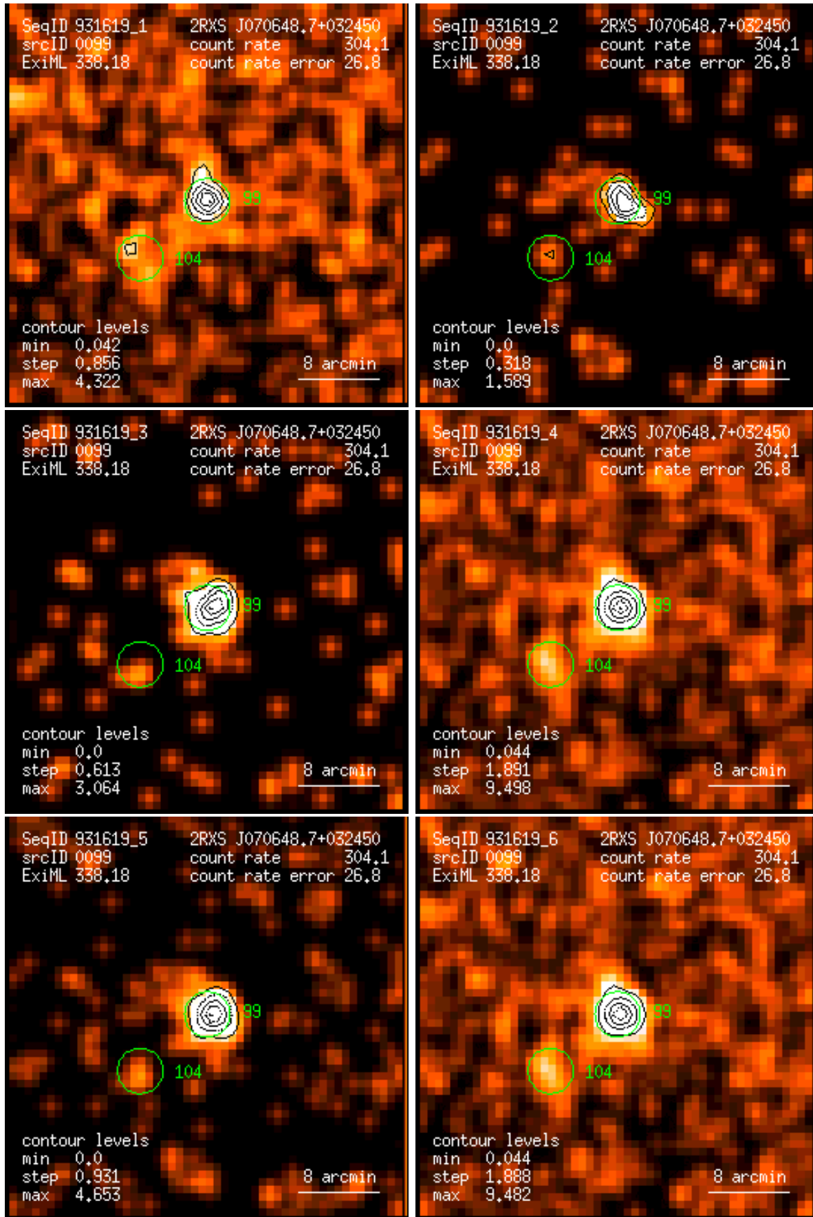
Figure 99: RASS 931619: detection 0099: band rate images, Gaussian filter: (1) PSPC channels 11 – 41, (2) 52 – 90, (3) 91 – 201, (4) 11 – 235, (5) 52 – 201, (6) 11 – 201. Broad band rates in counts/ks. Band rate contour levels in counts/ks/arcmin 2 .
