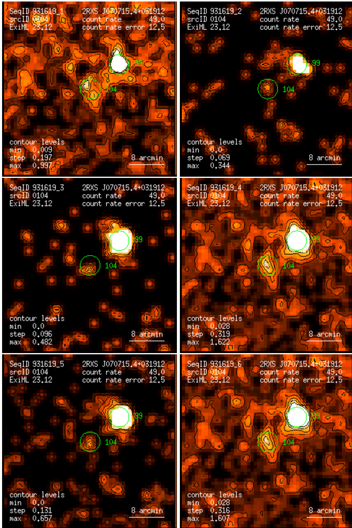
Figure 104: RASS 931619: detection 0104: band rate images, Gaussian filter: (1) PSPC channels 11 – 41, (2) 52 – 90, (3) 91 – 201, (4) 11 – 235, (5) 52 – 201, (6) 11 – 201. Broad band rates in counts/ks. Band rate contour levels in counts/ks/arcmin 2 .
