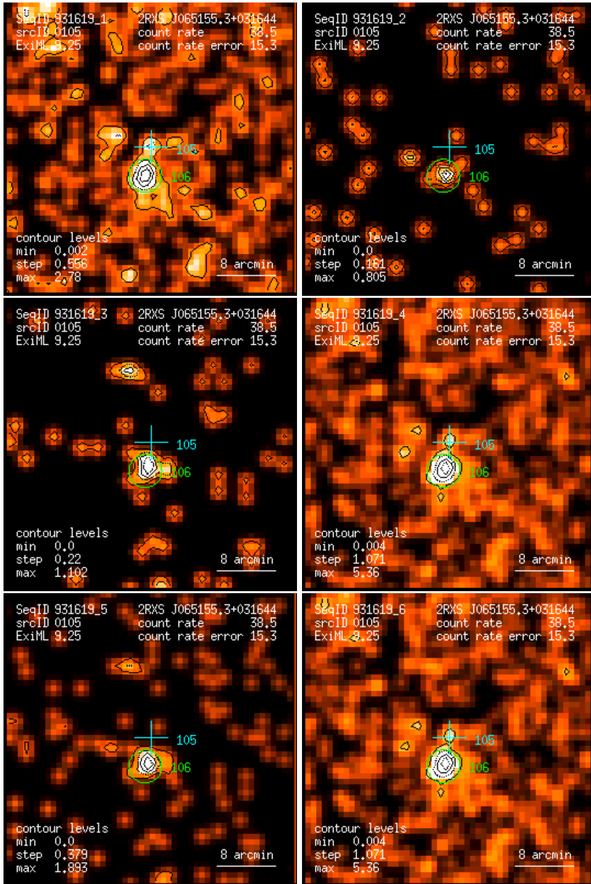
Figure 105: RASS 931619: detection 0105: band rate images, Gaussian filter: (1) PSPC channels 11 – 41, (2) 52 – 90, (3) 91 – 201, (4) 11 – 235, (5) 52 – 201, (6) 11 – 201. Broad band rates in counts/ks. Band rate contour levels in counts/ks/arcmin 2 .
