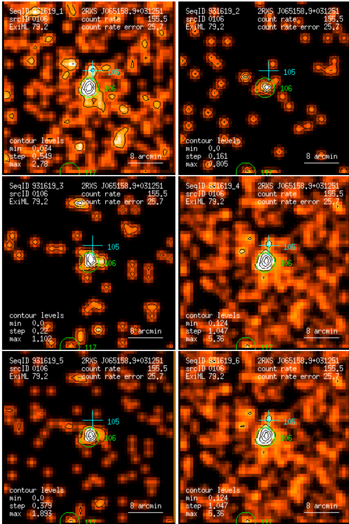
Figure 106: RASS 931619: detection 0106: band rate images, Gaussian filter: (1) PSPC channels 11 – 41, (2) 52 – 90, (3) 91 – 201, (4) 11 – 235, (5) 52 – 201, (6) 11 – 201. Broad band rates in counts/ks. Band rate contour levels in counts/ks/arcmin 2 .
