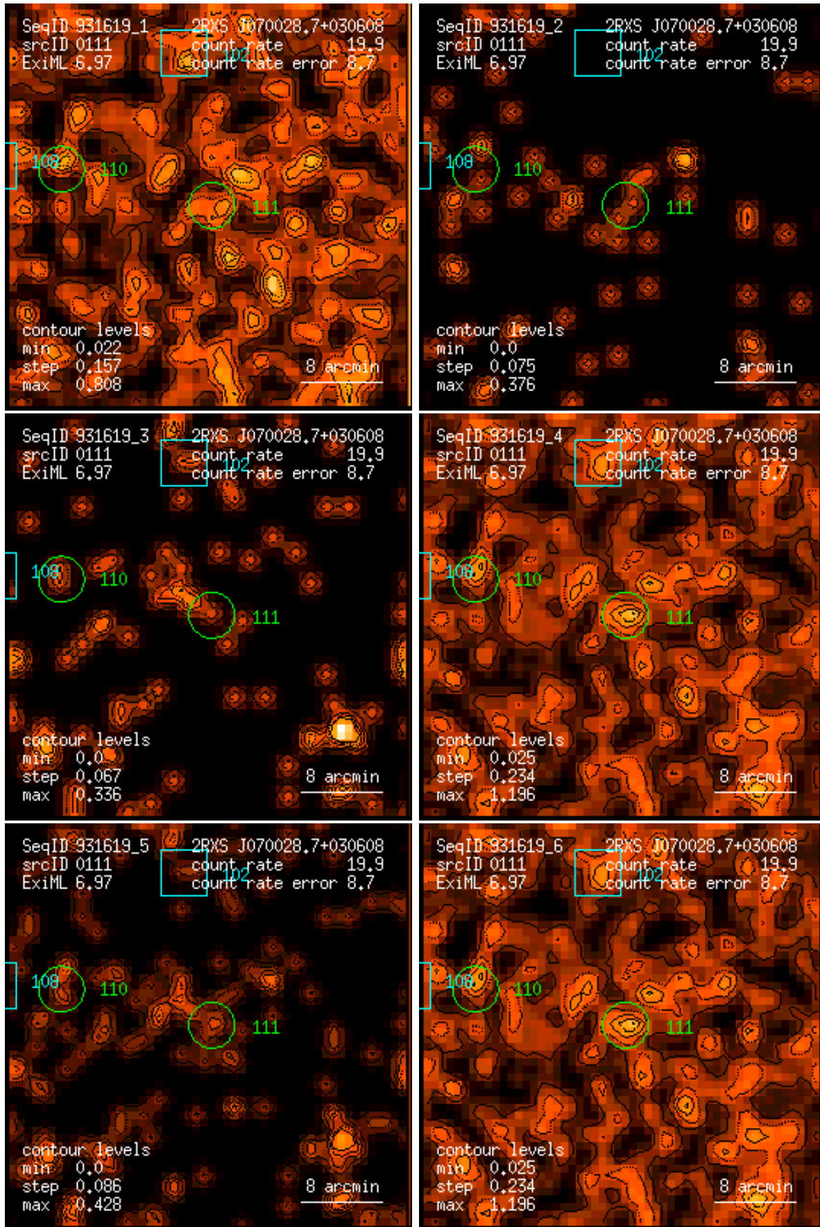
Figure 111: RASS 931619: detection 0111: band rate images, Gaussian filter: (1) PSPC channels 11 – 41, (2) 52 – 90, (3) 91 – 201, (4) 11 – 235, (5) 52 – 201, (6) 11 – 201. Broad band rates in counts/ks. Band rate contour levels in counts/ks/arcmin 2 .
