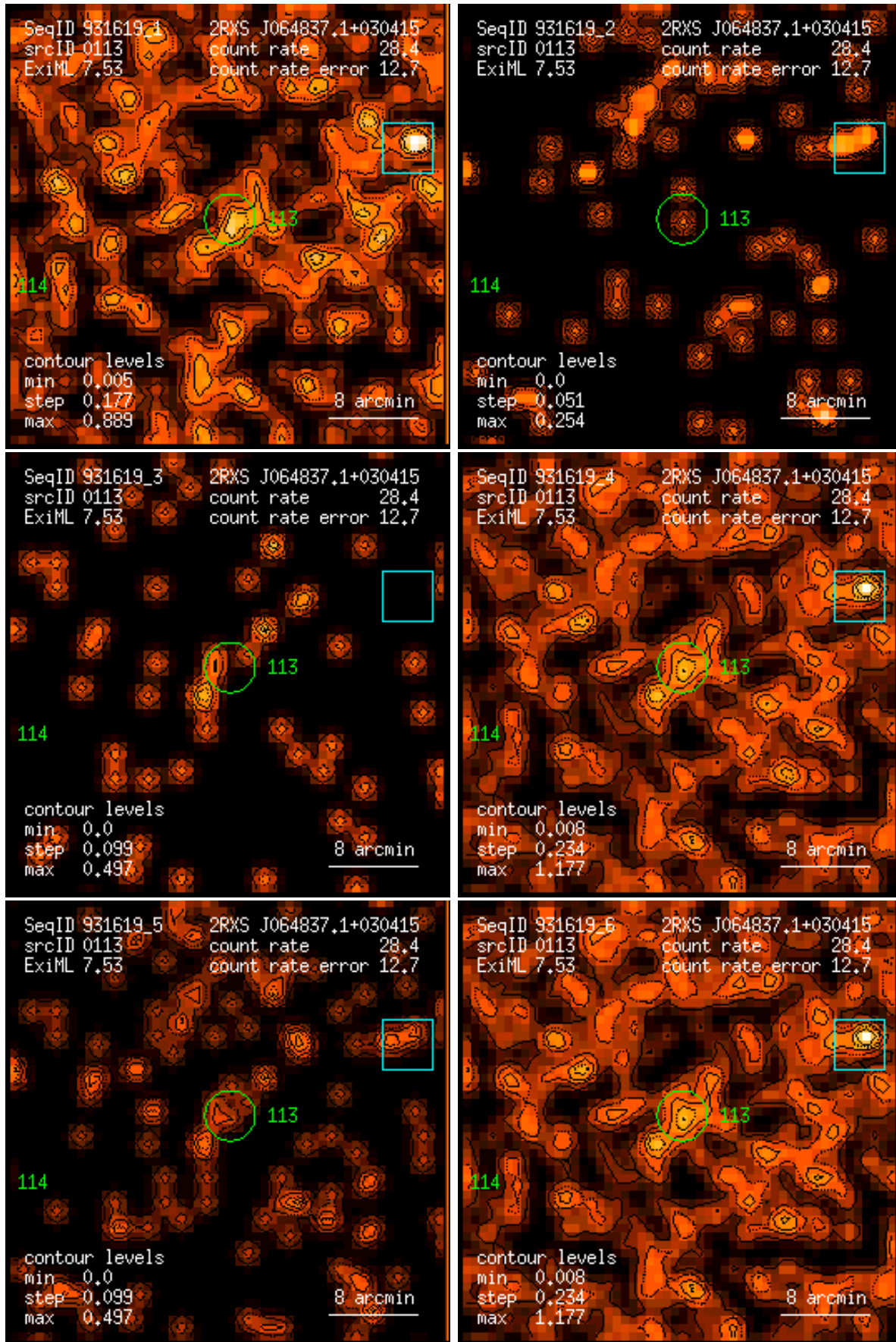
Figure 113: RASS 931619: detection 0113: band rate images, Gaussian filter: (1) PSPC channels 11 – 41, (2) 52 – 90, (3) 91 – 201, (4) 11 – 235, (5) 52 – 201, (6) 11 – 201. Broad band rates in counts/ks. Band rate contour levels in counts/ks/arcmin 2 .
