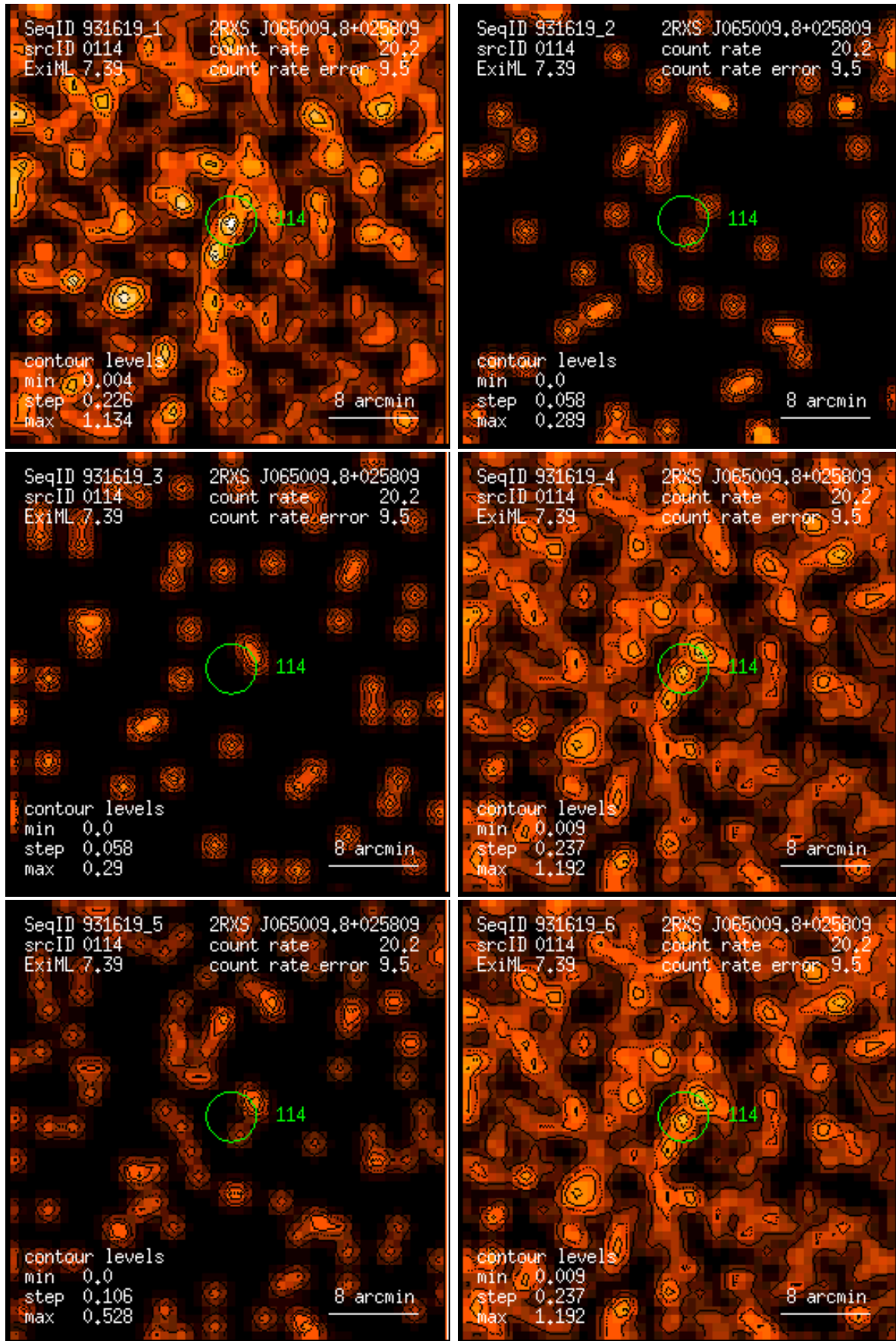
Figure 114: RASS 931619: detection 0114: band rate images, Gaussian filter: (1) PSPC channels 11 – 41, (2) 52 – 90, (3) 91 – 201, (4) 11 – 235, (5) 52 – 201, (6) 11 – 201. Broad band rates in counts/ks. Band rate contour levels in counts/ks/arcmin 2 .
