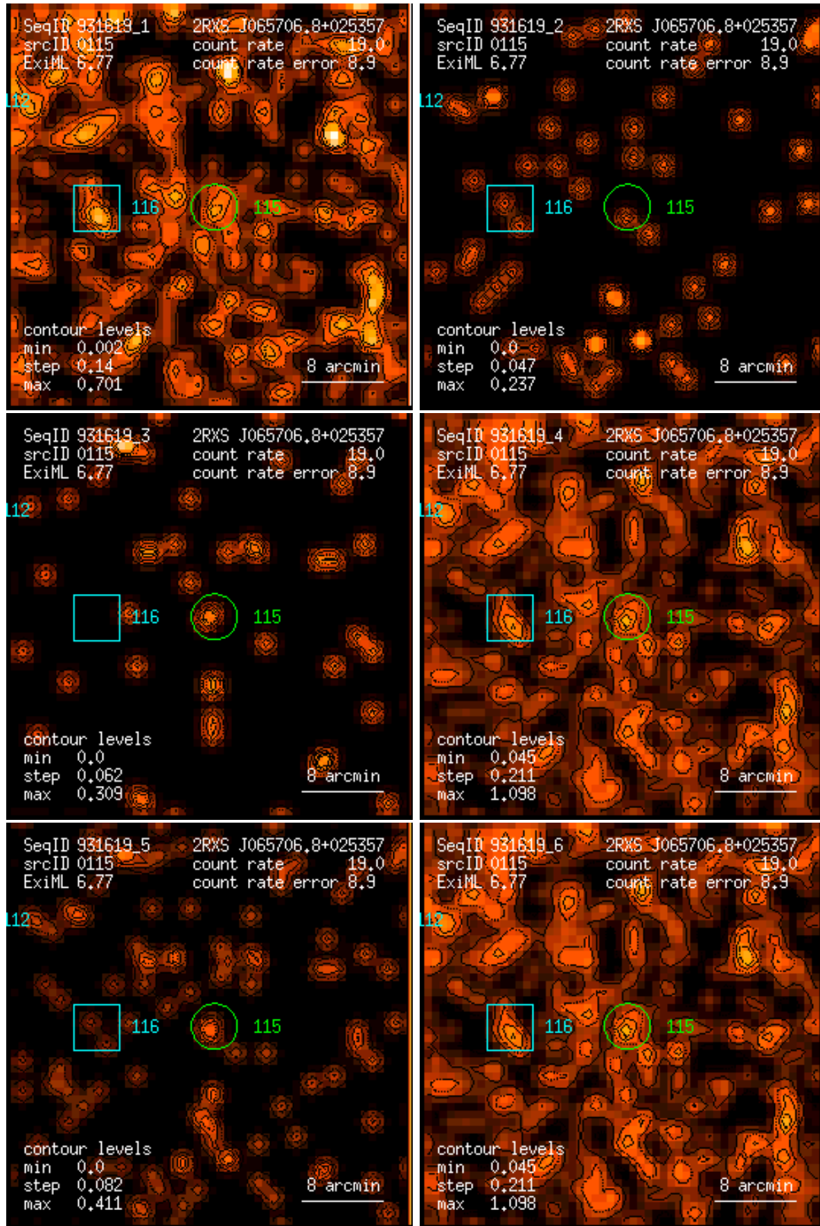
Figure 115: RASS 931619: detection 0115: band rate images, Gaussian filter: (1) PSPC channels 11 – 41, (2) 52 – 90, (3) 91 – 201, (4) 11 – 235, (5) 52 – 201, (6) 11 – 201. Broad band rates in counts/ks. Band rate contour levels in counts/ks/arcmin 2 .
