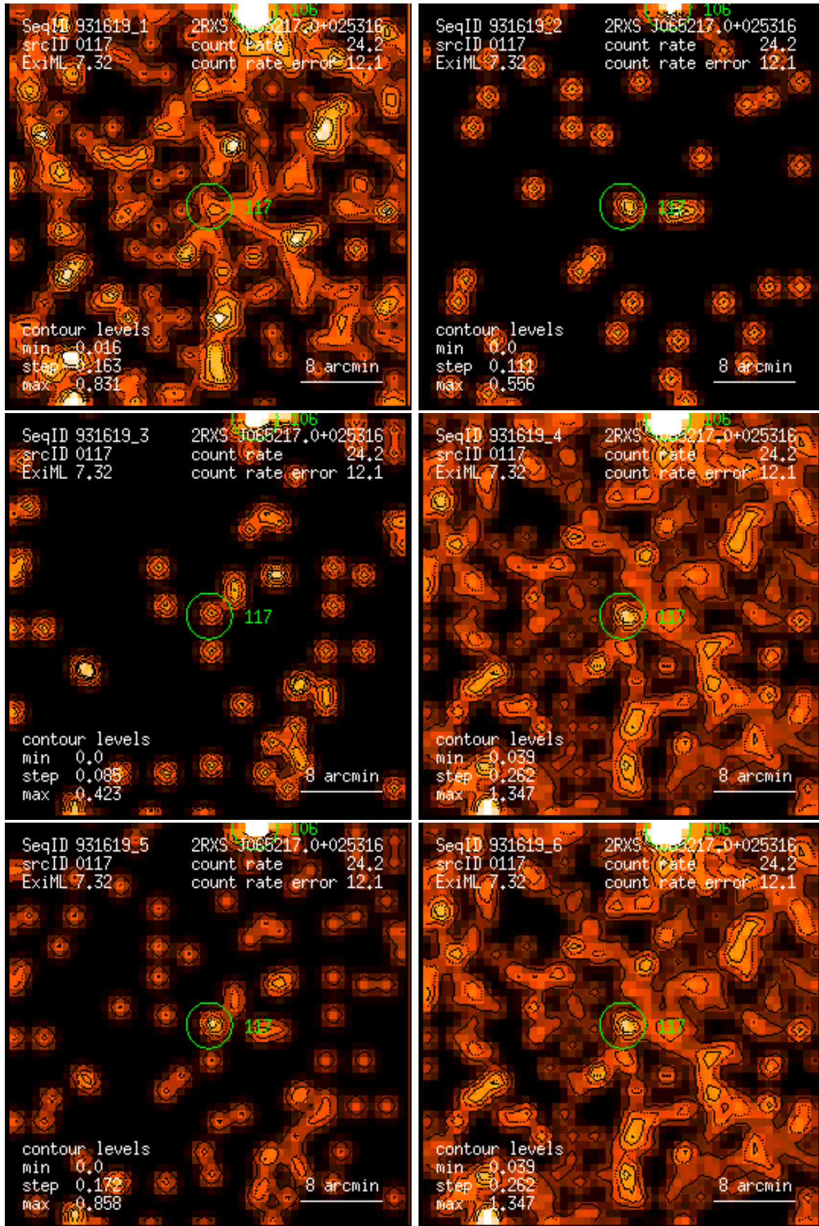
Figure 117: RASS 931619: detection 0117: band rate images, Gaussian filter: (1) PSPC channels 11 – 41, (2) 52 – 90, (3) 91 – 201, (4) 11 – 235, (5) 52 – 201, (6) 11 – 201. Broad band rates in counts/ks. Band rate contour levels in counts/ks/arcmin 2 .
