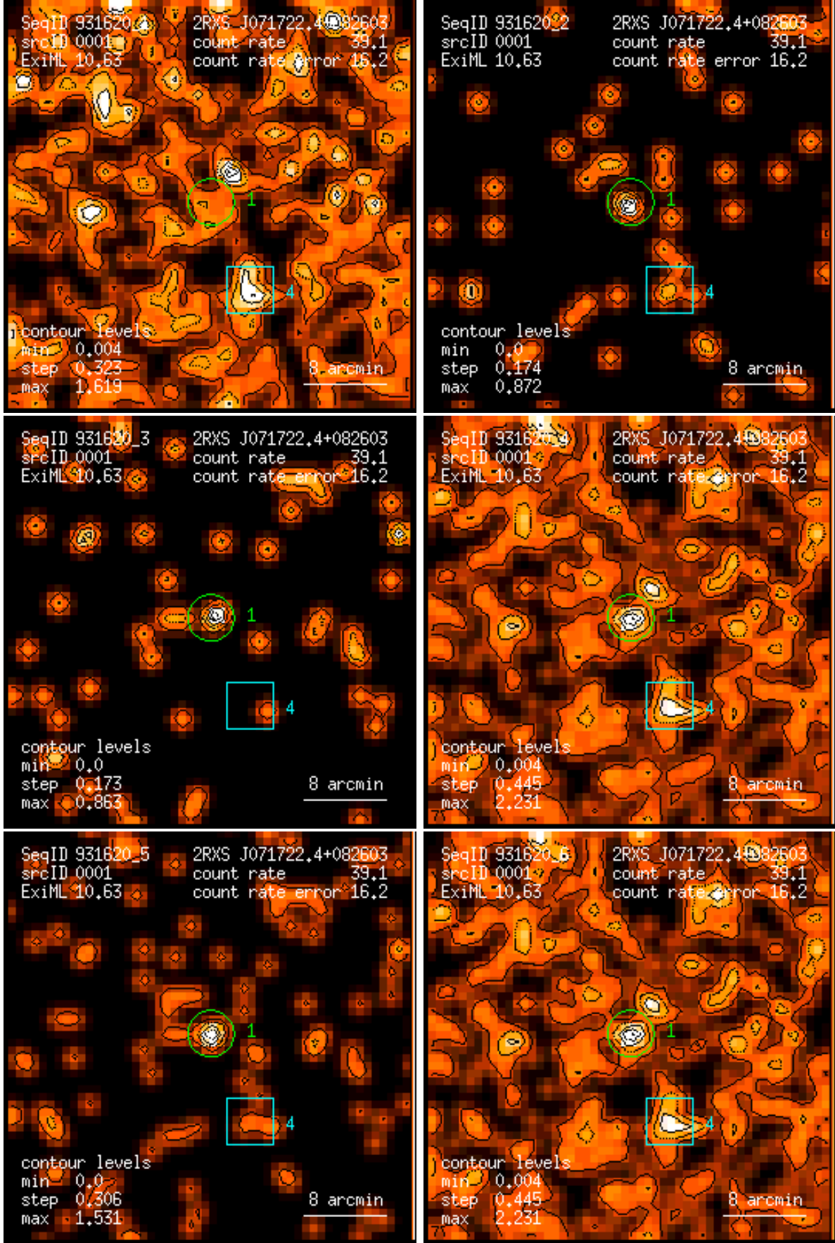
Figure 1: RASS 931620: detection 0001: band rate images, Gaussian filter: (1) PSPC channels 11 – 41, (2) 52 – 90, (3) 91 – 201, (4) 11 – 235, (5) 52 – 201, (6) 11 – 201. Broad band rates in counts/ks. Band rate contour levels in counts/ks/arcmin 2 .
