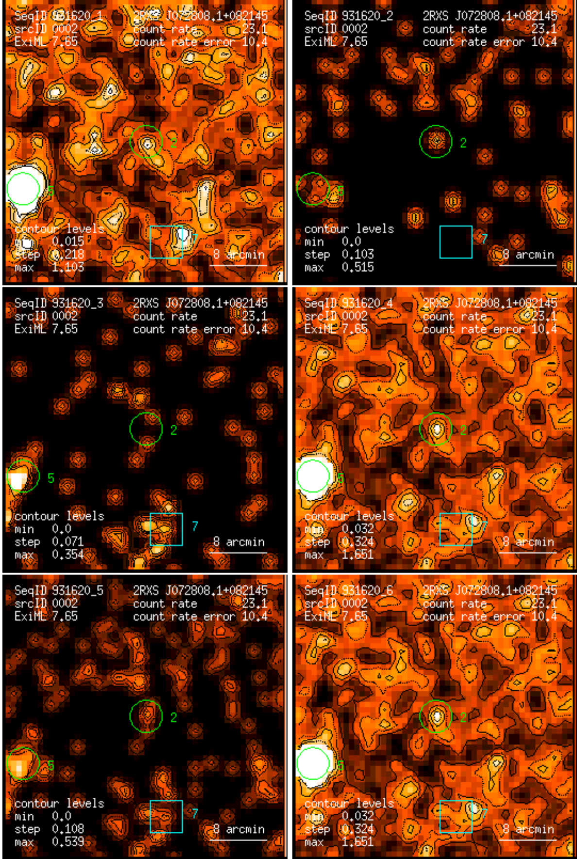
Figure 2: RASS 931620: detection 0002: band rate images, Gaussian filter: (1) PSPC channels 11 – 41, (2) 52 – 90, (3) 91 – 201, (4) 11 – 235, (5) 52 – 201, (6) 11 – 201. Broad band rates in counts/ks. Band rate contour levels in counts/ks/arcmin 2 .
