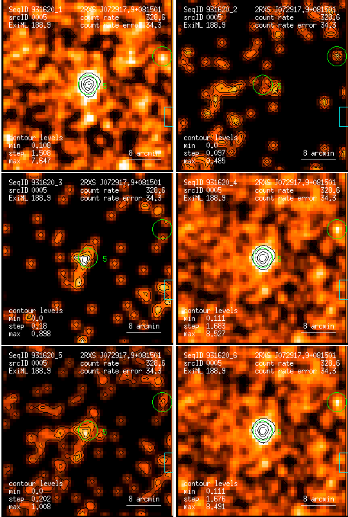
Figure 5: RASS 931620: detection 0005: band rate images, Gaussian filter: (1) PSPC channels 11 – 41, (2) 52 – 90, (3) 91 – 201, (4) 11 – 235, (5) 52 – 201, (6) 11 – 201. Broad band rates in counts/ks. Band rate contour levels in counts/ks/arcmin 2 .
