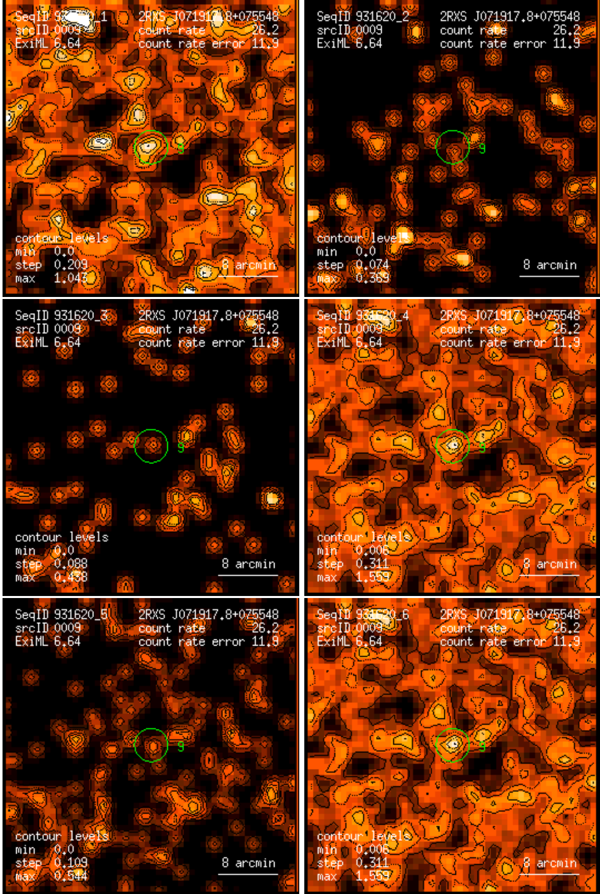
Figure 9: RASS 931620: detection 0009: band rate images, Gaussian filter: (1) PSPC channels 11 – 41, (2) 52 – 90, (3) 91 – 201, (4) 11 – 235, (5) 52 – 201, (6) 11 – 201. Broad band rates in counts/ks. Band rate contour levels in counts/ks/arcmin 2 .
