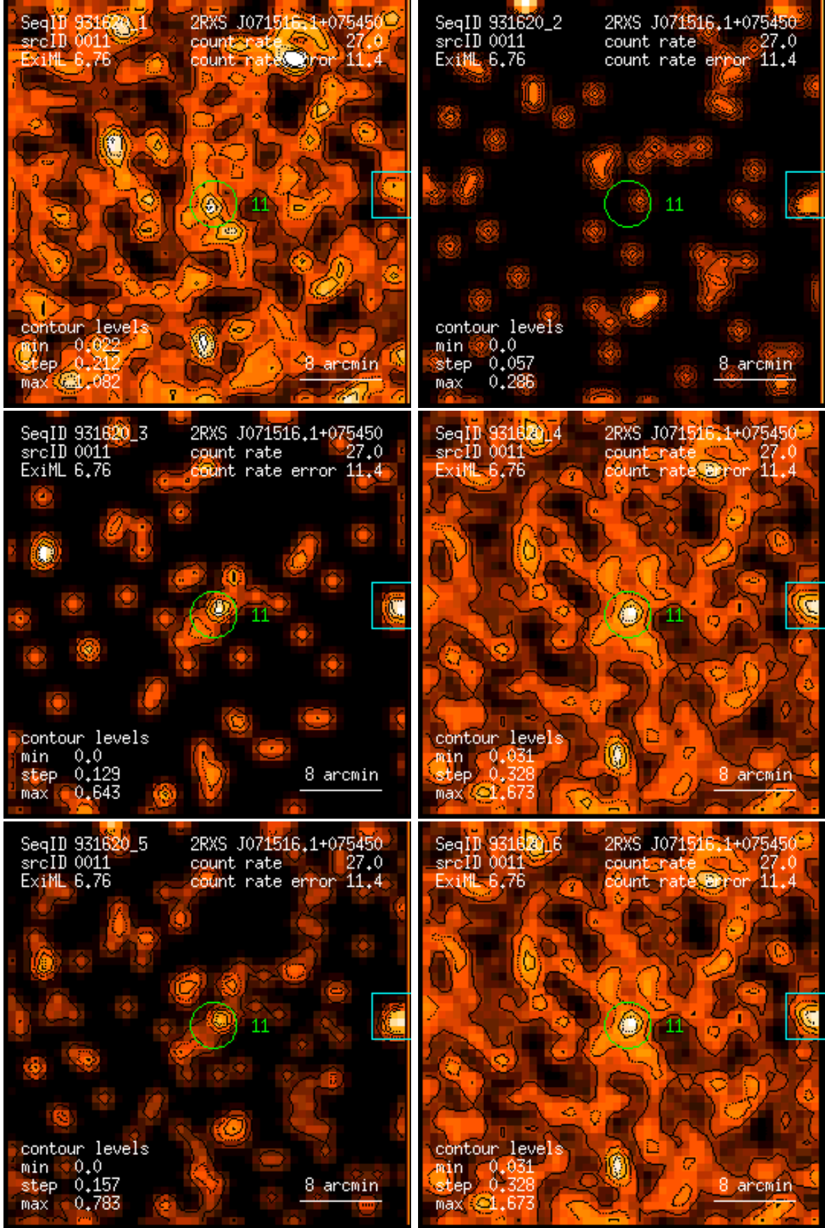
Figure 11: RASS 931620: detection 0011: band rate images, Gaussian filter: (1) PSPC channels 11 – 41, (2) 52 – 90, (3) 91 – 201, (4) 11 – 235, (5) 52 – 201, (6) 11 – 201. Broad band rates in counts/ks. Band rate contour levels in counts/ks/arcmin 2 .
