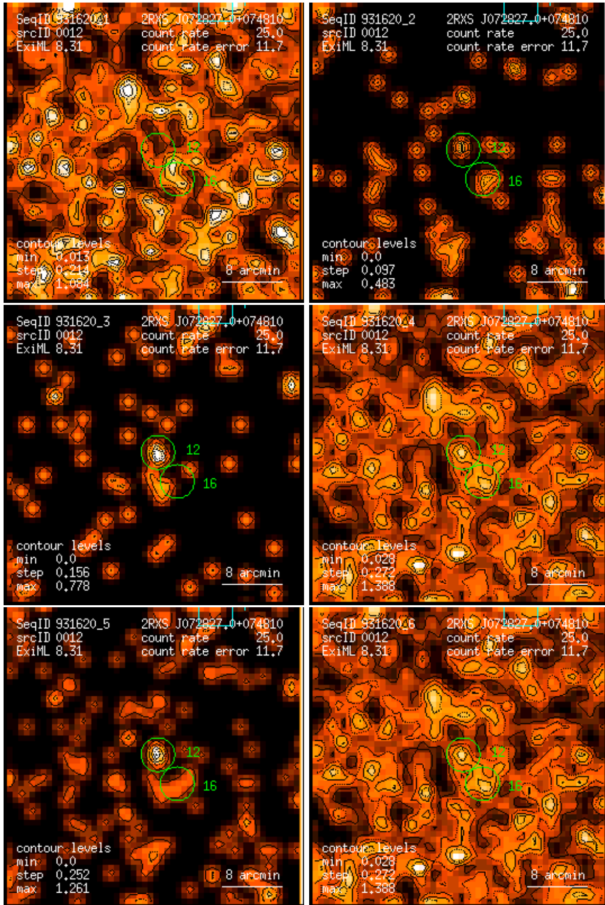
Figure 12: RASS 931620: detection 0012: band rate images, Gaussian filter: (1) PSPC channels 11 – 41, (2) 52 – 90, (3) 91 – 201, (4) 11 – 235, (5) 52 – 201, (6) 11 – 201. Broad band rates in counts/ks. Band rate contour levels in counts/ks/arcmin 2 .
