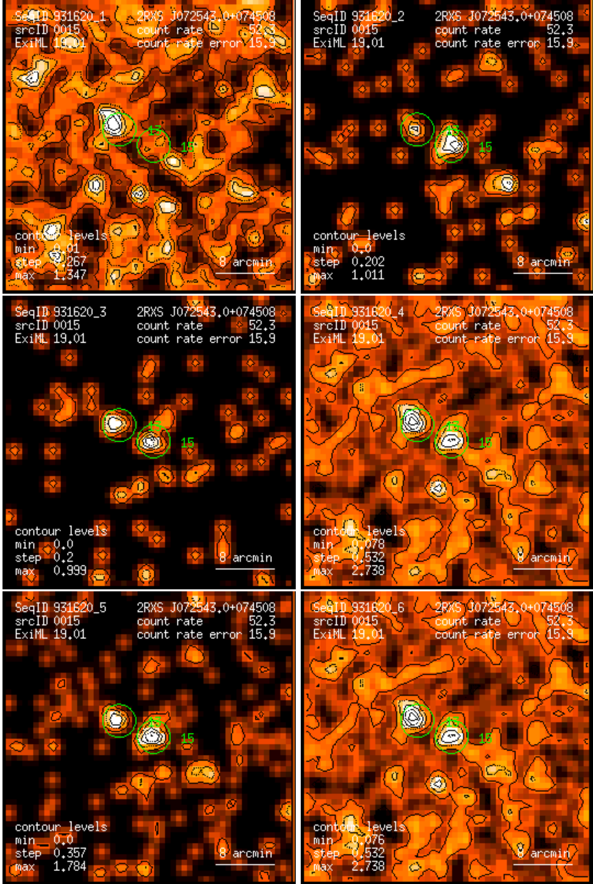
Figure 15: RASS 931620: detection 0015: band rate images, Gaussian filter: (1) PSPC channels 11 – 41, (2) 52 – 90, (3) 91 – 201, (4) 11 – 235, (5) 52 – 201, (6) 11 – 201. Broad band rates in counts/ks. Band rate contour levels in counts/ks/arcmin 2 .
