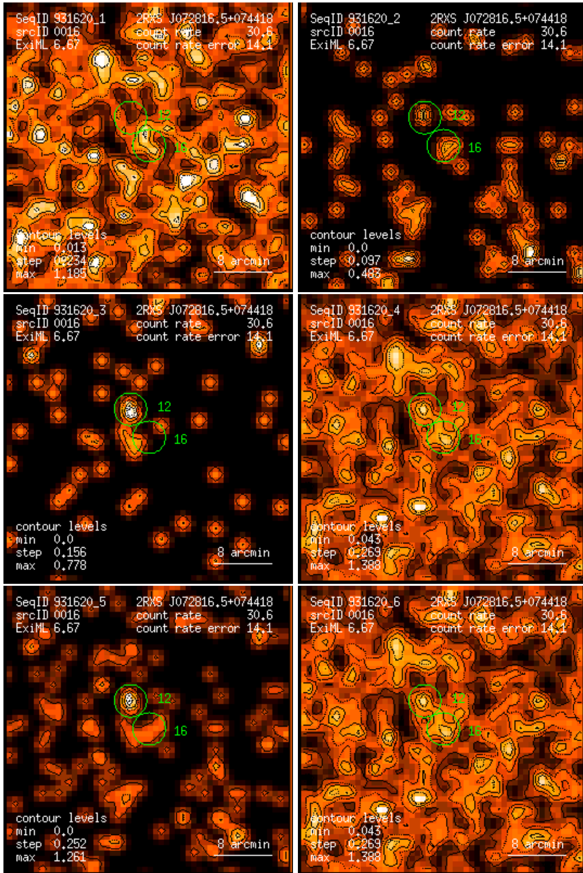
Figure 16: RASS 931620: detection 0016: band rate images, Gaussian filter: (1) PSPC channels 11 – 41, (2) 52 – 90, (3) 91 – 201, (4) 11 – 235, (5) 52 – 201, (6) 11 – 201. Broad band rates in counts/ks. Band rate contour levels in counts/ks/arcmin 2 .
