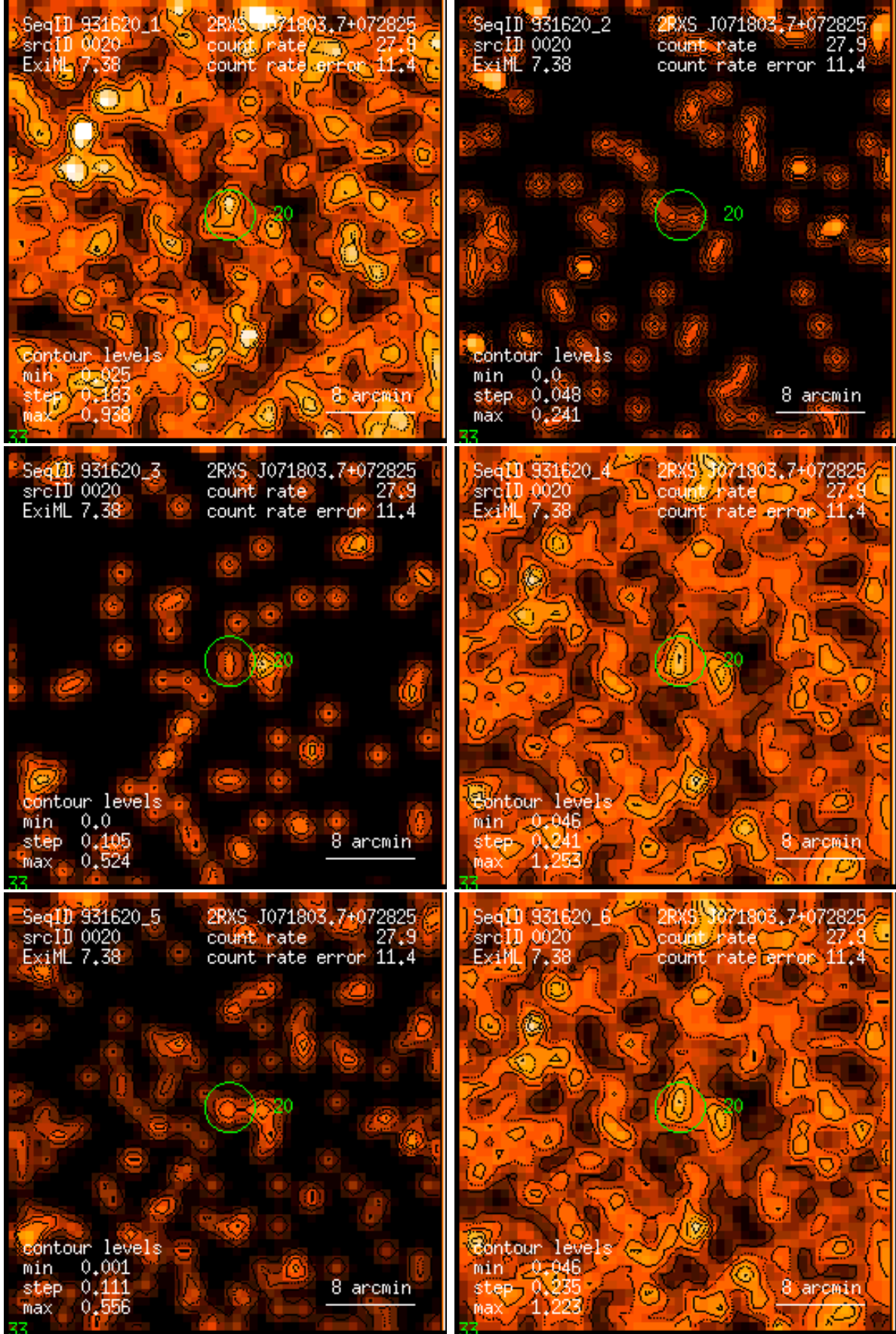
Figure 20: RASS 931620: detection 0020: band rate images, Gaussian filter: (1) PSPC channels 11 – 41, (2) 52 – 90, (3) 91 – 201, (4) 11 – 235, (5) 52 – 201, (6) 11 – 201. Broad band rates in counts/ks. Band rate contour levels in counts/ks/arcmin 2 .
