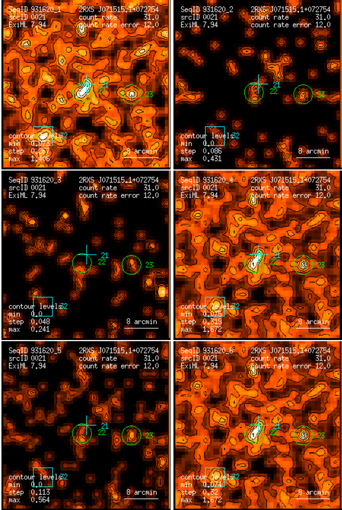
Figure 21: RASS 931620: detection 0021: band rate images, Gaussian filter: (1) PSPC channels 11 – 41, (2) 52 – 90, (3) 91 – 201, (4) 11 – 235, (5) 52 – 201, (6) 11 – 201. Broad band rates in counts/ks. Band rate contour levels in counts/ks/arcmin 2 .
