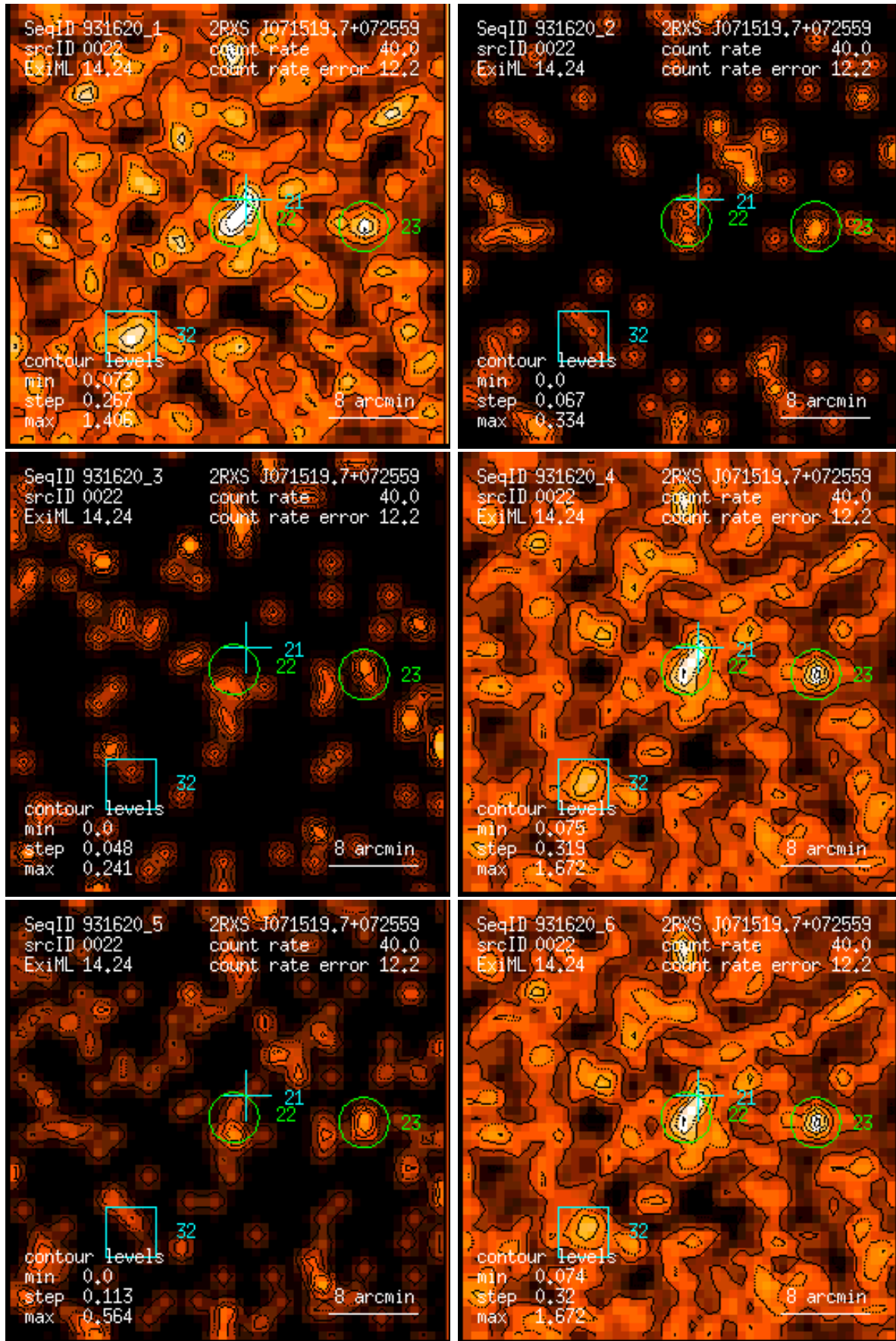
Figure 22: RASS 931620: detection 0022: band rate images, Gaussian filter: (1) PSPC channels 11 – 41, (2) 52 – 90, (3) 91 – 201, (4) 11 – 235, (5) 52 – 201, (6) 11 – 201. Broad band rates in counts/ks. Band rate contour levels in counts/ks/arcmin 2 .
