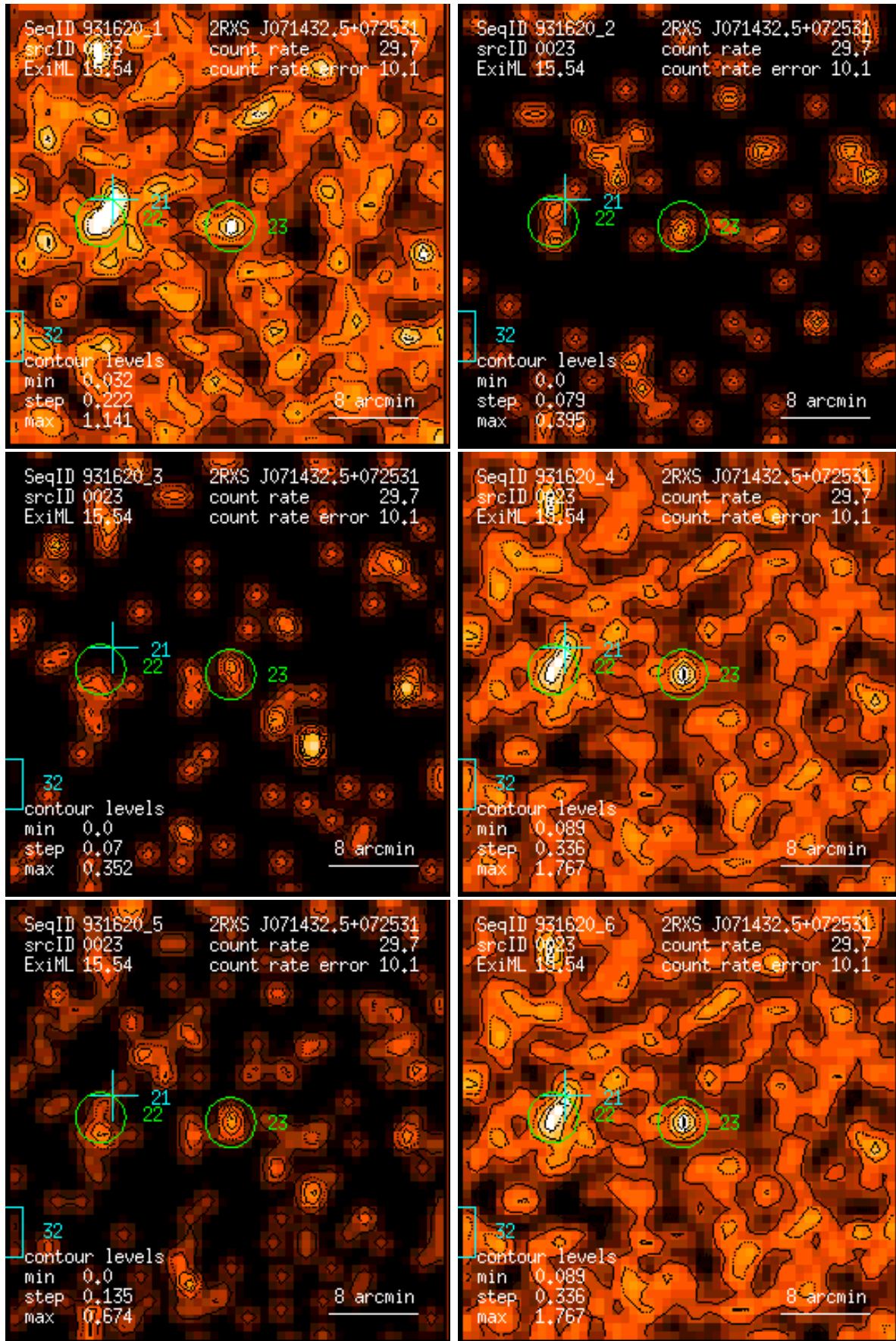
Figure 23: RASS 931620: detection 0023: band rate images, Gaussian filter: (1) PSPC channels 11 – 41, (2) 52 – 90, (3) 91 – 201, (4) 11 – 235, (5) 52 – 201, (6) 11 – 201. Broad band rates in counts/ks. Band rate contour levels in counts/ks/arcmin 2 .
