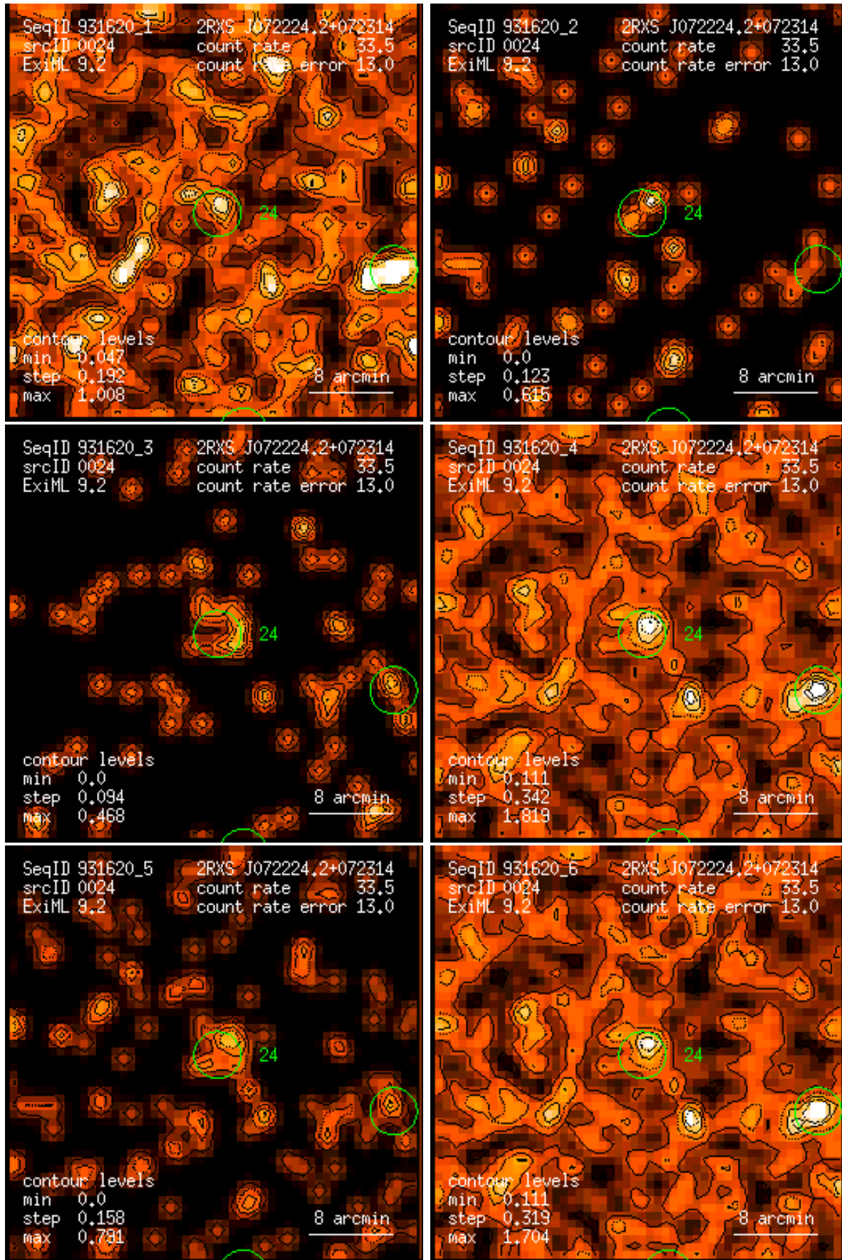
Figure 24: RASS 931620: detection 0024: band rate images, Gaussian filter: (1) PSPC channels 11 – 41, (2) 52 – 90, (3) 91 – 201, (4) 11 – 235, (5) 52 – 201, (6) 11 – 201. Broad band rates in counts/ks. Band rate contour levels in counts/ks/arcmin 2 .
