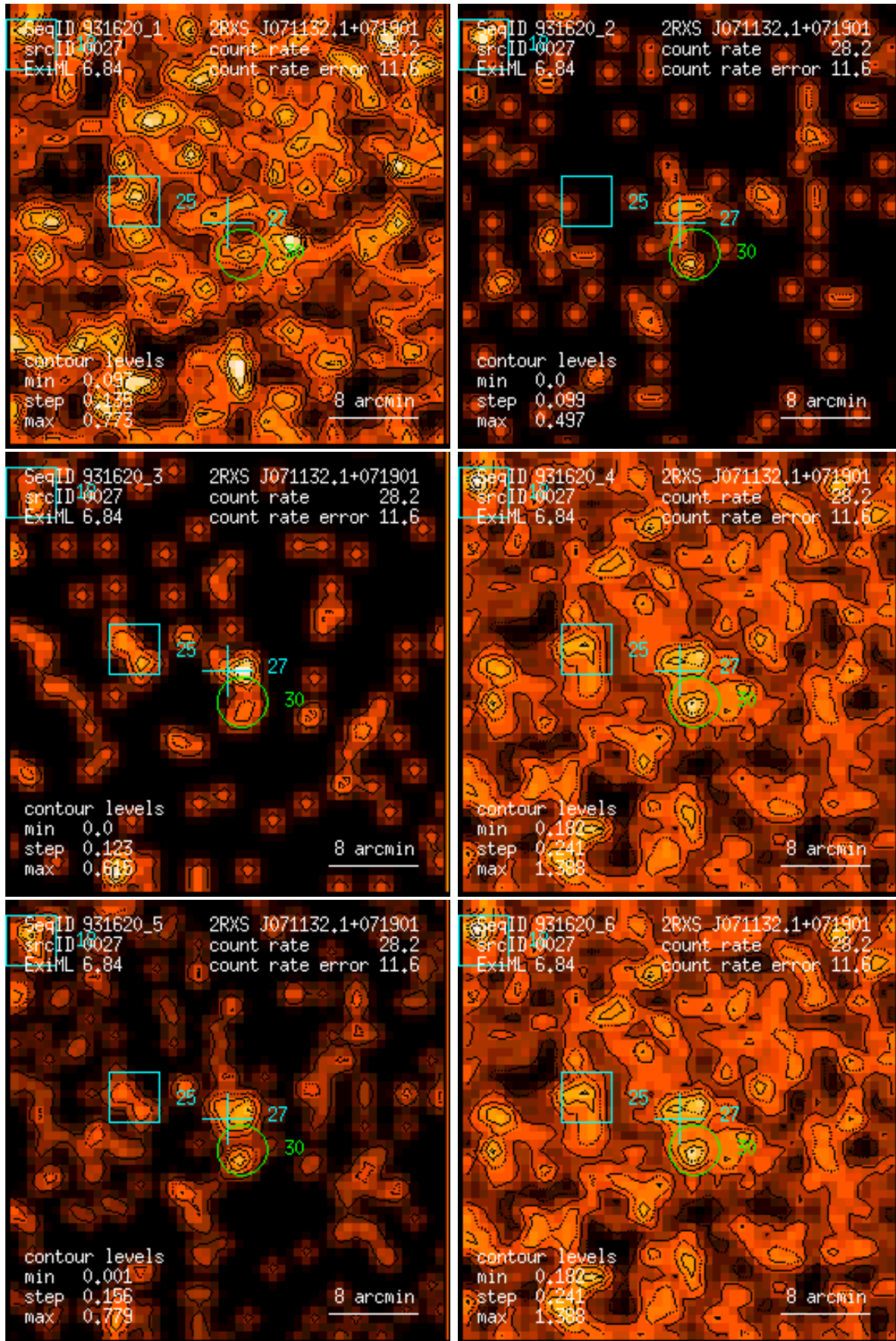
Figure 27: RASS 931620: detection 0027: band rate images, Gaussian filter: (1) PSPC channels 11 – 41, (2) 52 – 90, (3) 91 – 201, (4) 11 – 235, (5) 52 – 201, (6) 11 – 201. Broad band rates in counts/ks. Band rate contour levels in counts/ks/arcmin 2 .
