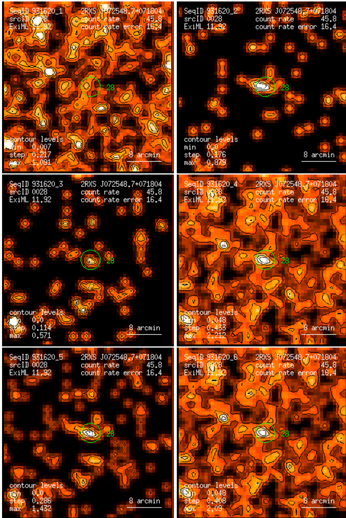
Figure 28: RASS 931620: detection 0028: band rate images, Gaussian filter: (1) PSPC channels 11 – 41, (2) 52 – 90, (3) 91 – 201, (4) 11 – 235, (5) 52 – 201, (6) 11 – 201. Broad band rates in counts/ks. Band rate contour levels in counts/ks/arcmin 2 .
