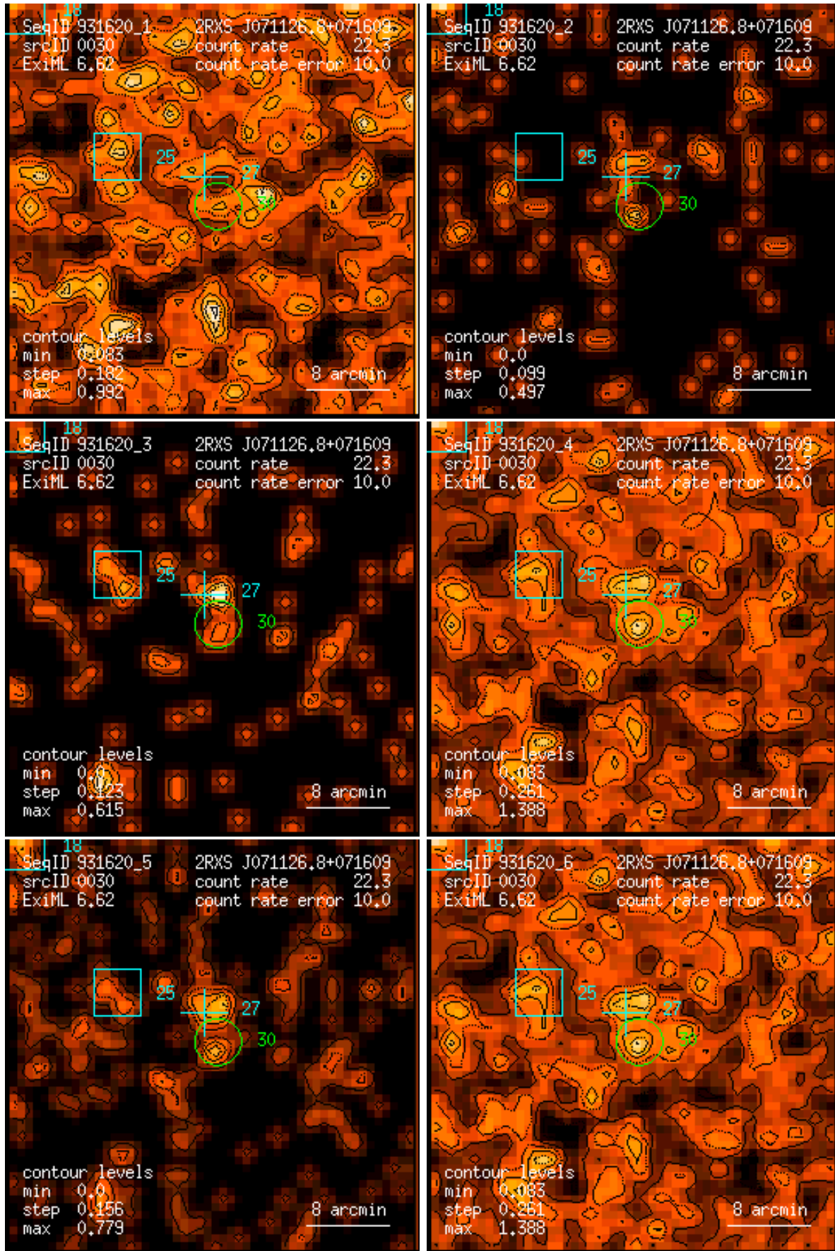
Figure 30: RASS 931620: detection 0030: band rate images, Gaussian filter: (1) PSPC channels 11 – 41, (2) 52 – 90, (3) 91 – 201, (4) 11 – 235, (5) 52 – 201, (6) 11 – 201. Broad band rates in counts/ks. Band rate contour levels in counts/ks/arcmin 2 .
