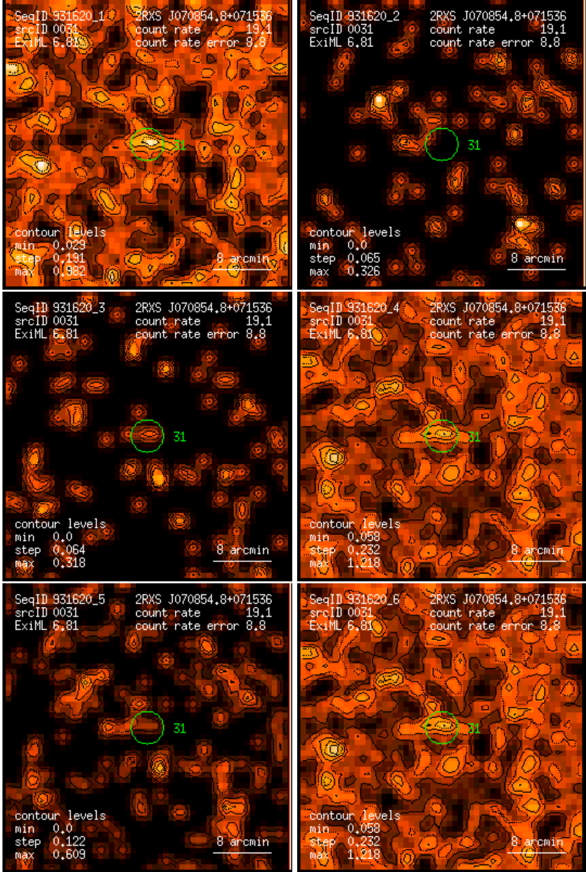
Figure 31: RASS 931620: detection 0031: band rate images, Gaussian filter: (1) PSPC channels 11 – 41, (2) 52 – 90, (3) 91 – 201, (4) 11 – 235, (5) 52 – 201, (6) 11 – 201. Broad band rates in counts/ks. Band rate contour levels in counts/ks/arcmin 2 .
